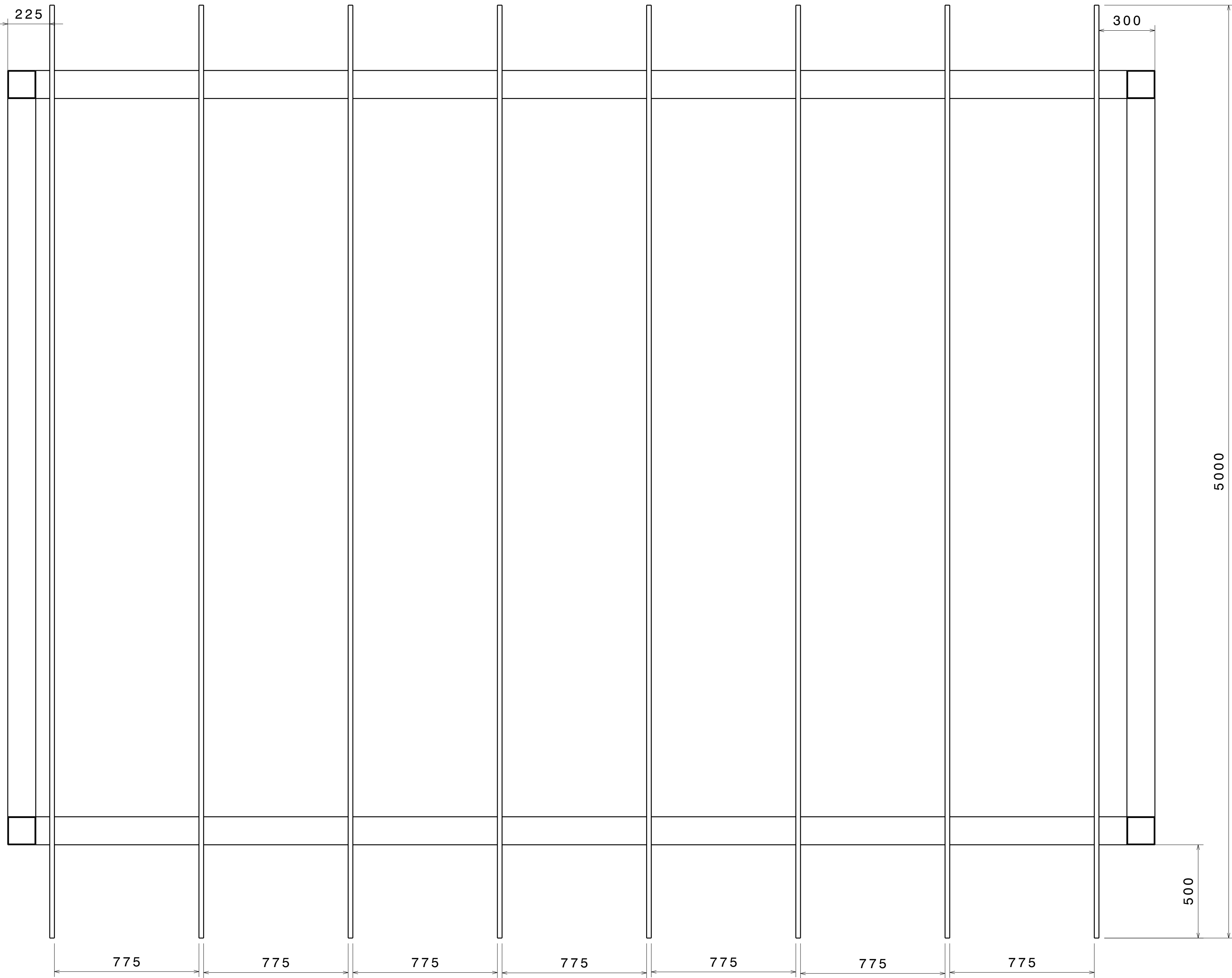
Top view
