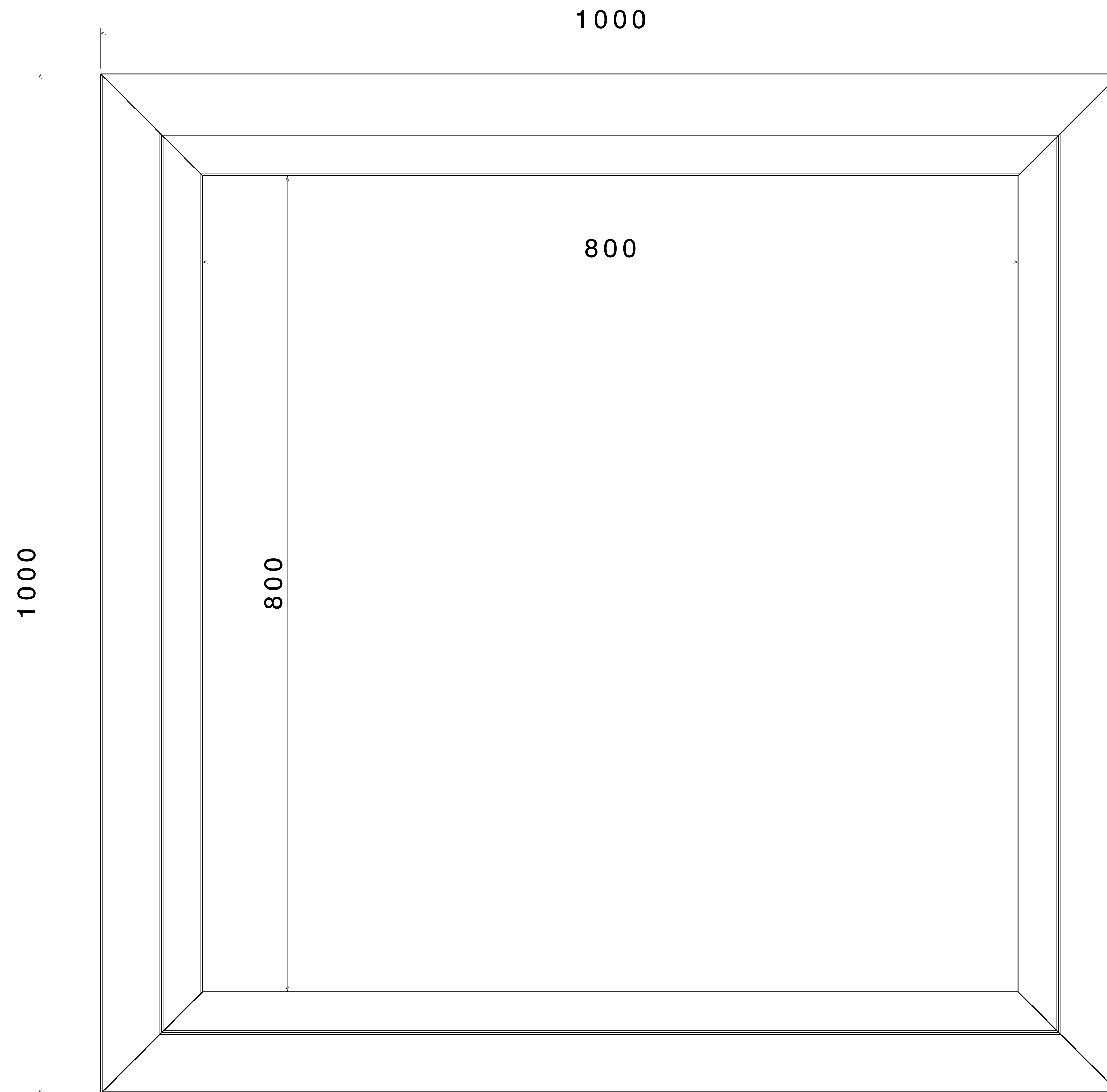
Front view Scale: 2:5
