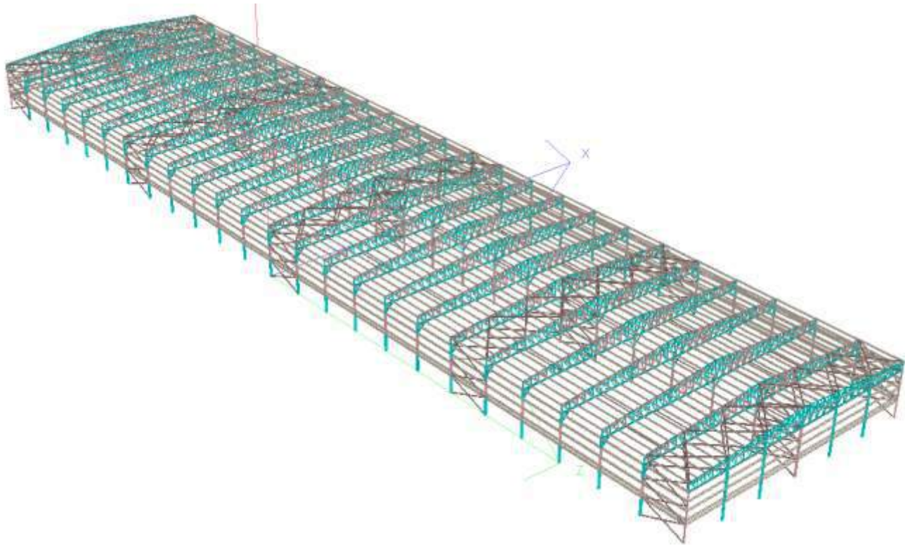
ISOMETRIC VIEW
