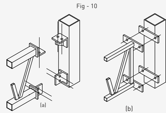
Figure 10(a&b) - Truss to SHS/RHS column connection
