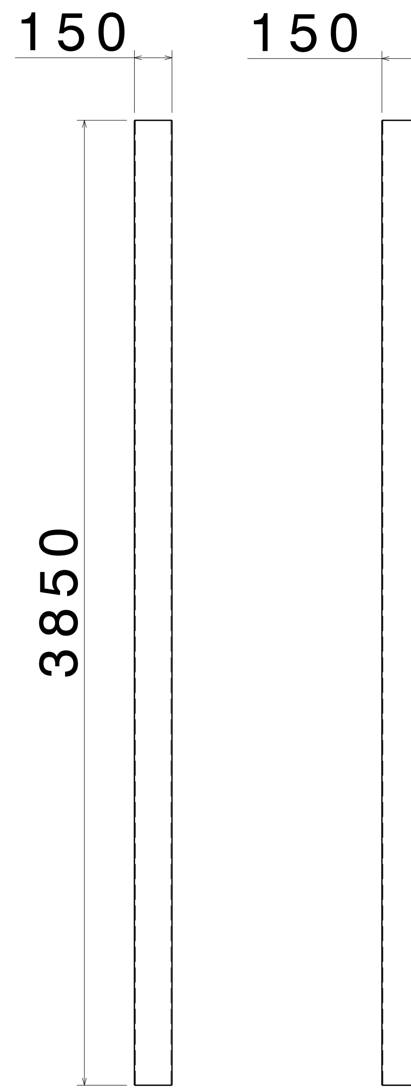
FRONT VIEW RIGHT VIEW SCALE: 1:15 SCALE: 1:15 ITEM 4, SHS FRAME 3 THICKNESS - 4.0 MM
