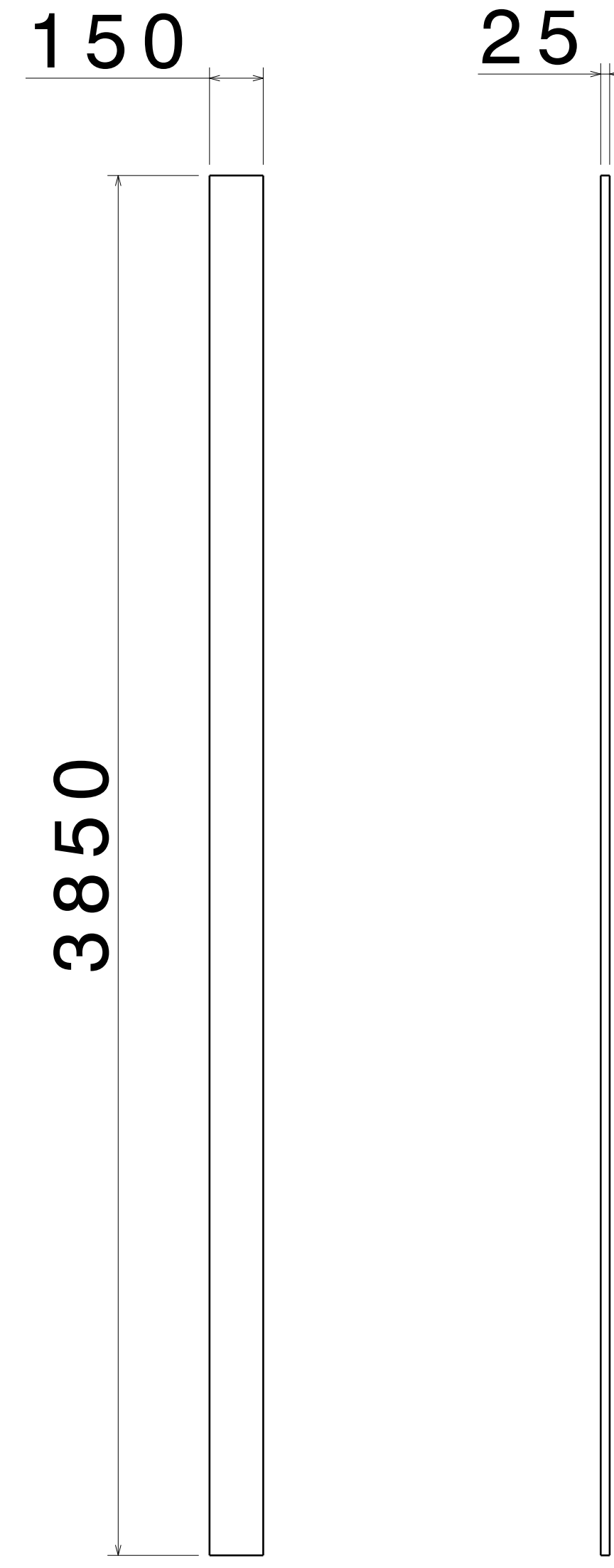
FRONT VIEW RIGHT VIEW SCALE: 1:15 SCALE: 1:15 ITEM 3, RHS PLANK 1 THICKNESS -1.6 MM
