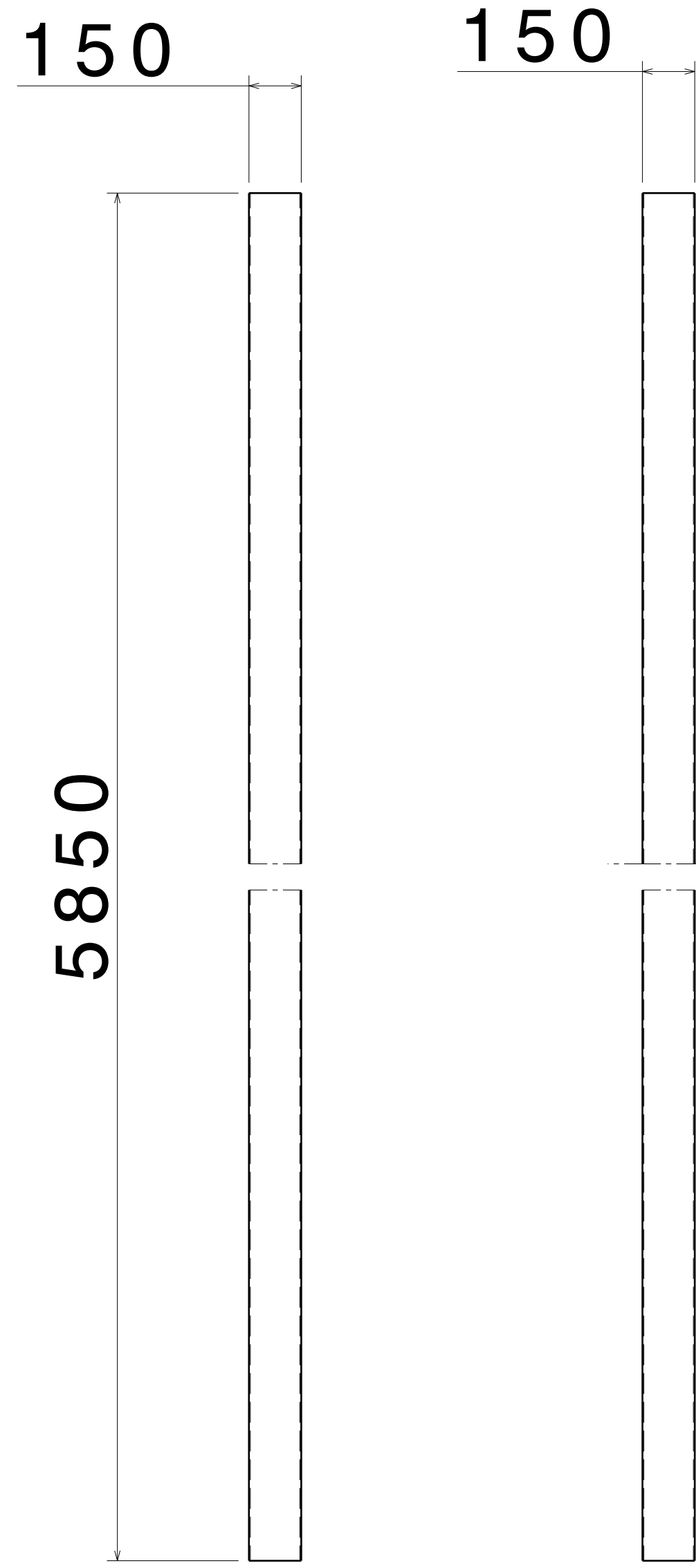
FRONT VIEW RIGHT VIEW SCALE: 1:15 SCALE: 1:15 ITEM 2, SHS FRAME 2 THICKNESS - 4.0 MM
