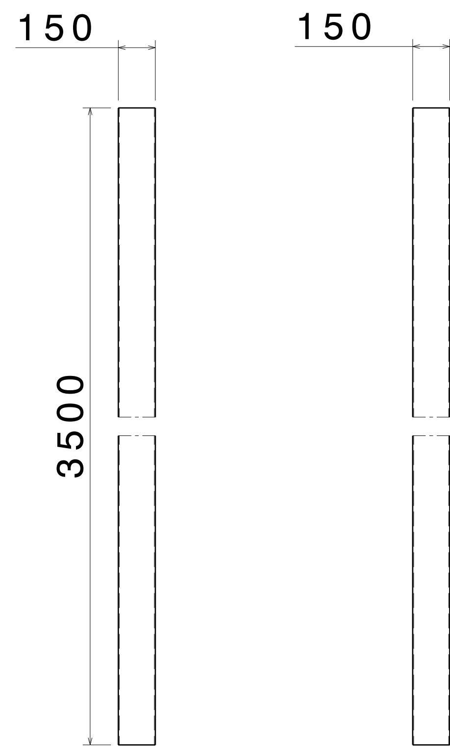
FRONT VIEW RIGHT VIEW SCALE: 1:15 SCALE: 1:15 ITEM 1, SHS FRAME 1 THICKNESS - 4.0MM
