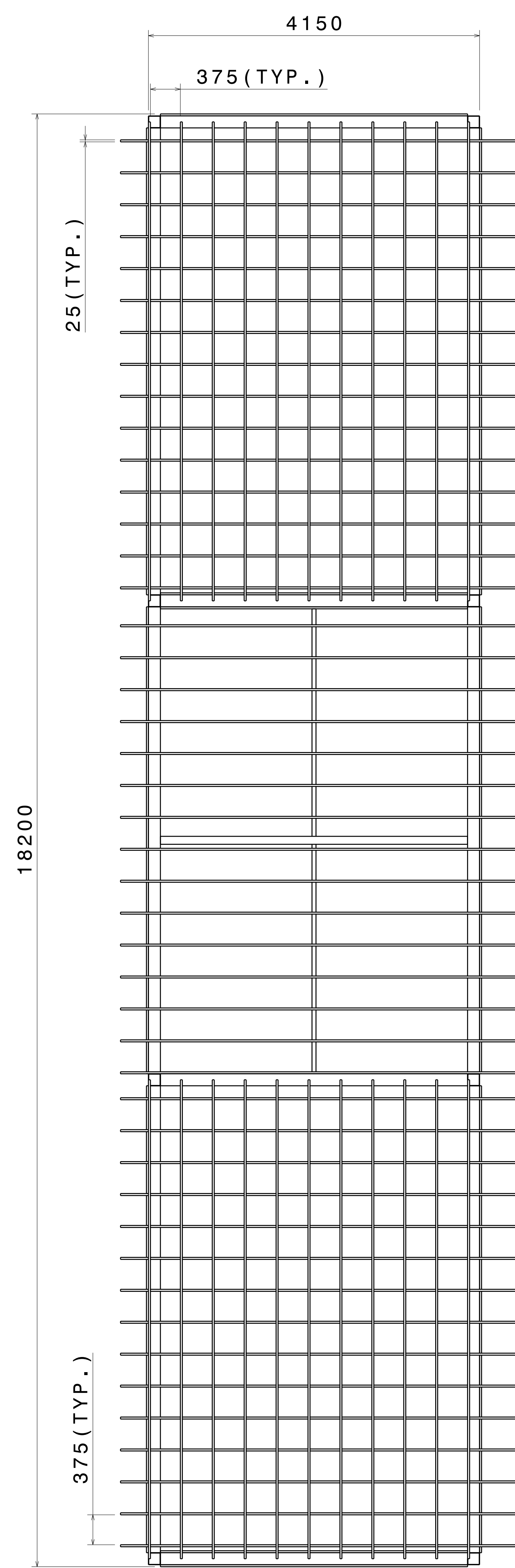
FRONT VIEW
