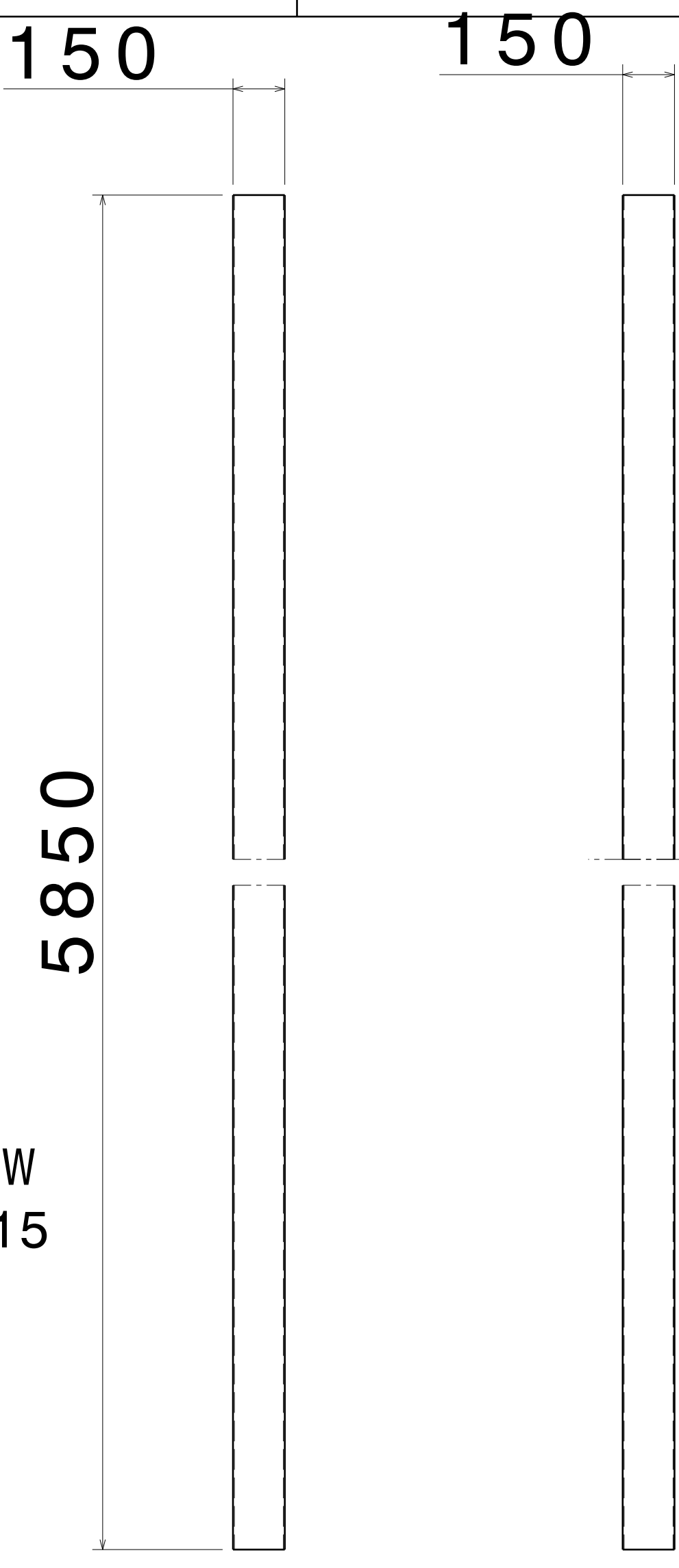
FRONT VIEW RIGHT VIEW SCALE: 1:15 SCALE: 1:15 ITEM 2, SHS FRAME 2 THICKNESS - 4.0 MM
