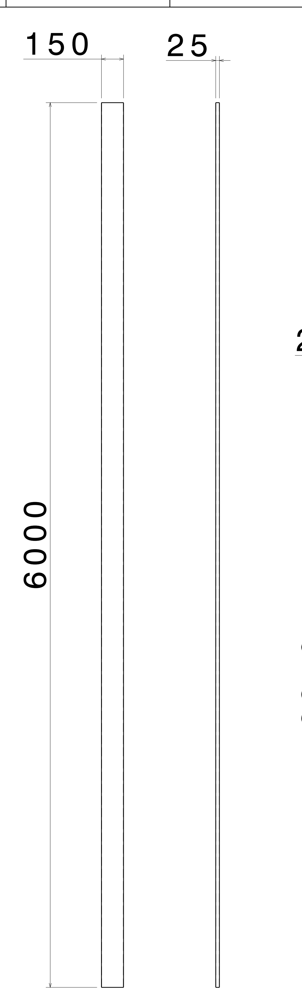
FRONT VIEW RIGHT VIEW SCALE: 1:15 SCALE: 1:15 ITEM 6, RHS PLANK 3 THICKNESS -1.6 MM
