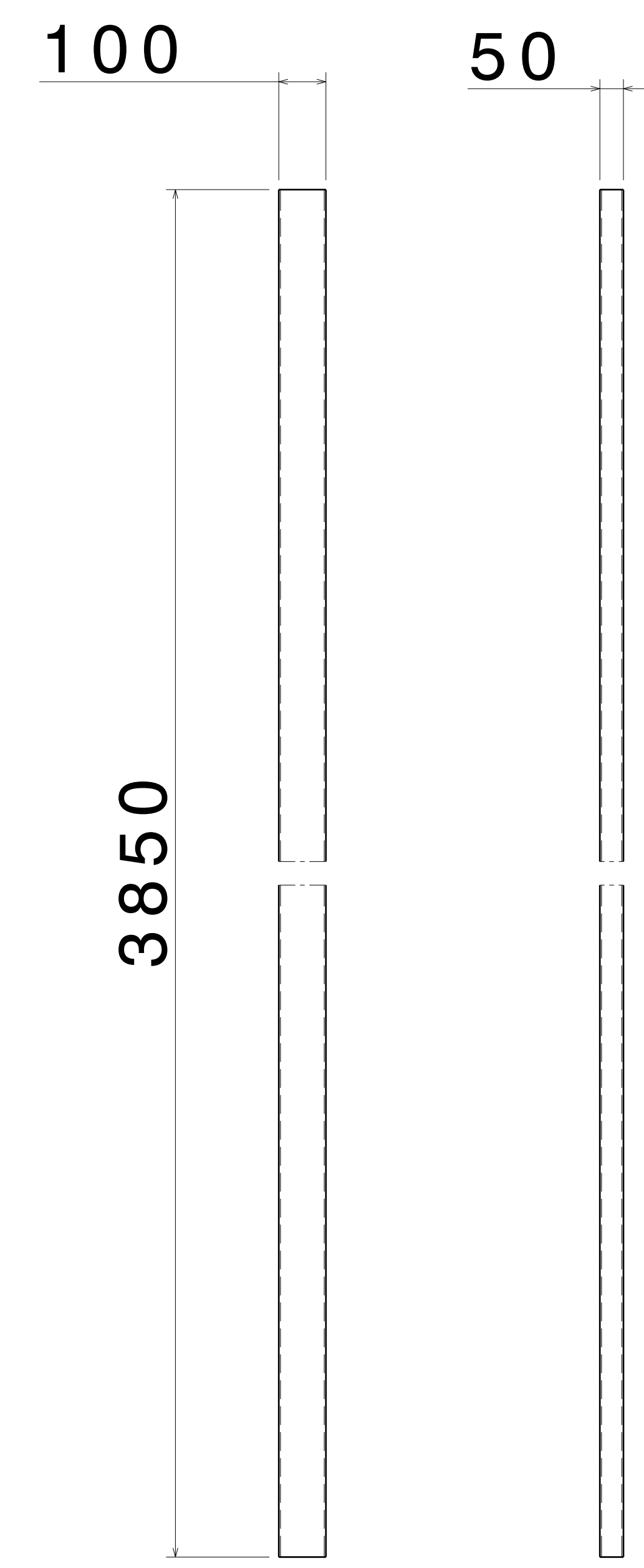
FRONT VIEW RIGHT VIEW SCALE: 1:15 SCALE: 1:15 ITEM 9, RHS FRAME 2 THICKNESS -3.6 MM
