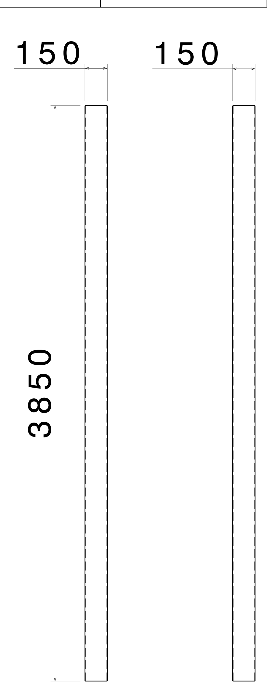
FRONT VIEW RIGHT VIEW SCALE: 1:15 SCALE: 1:15 ITEM 4, SHS FRAME 3 THICKNESS - 4.0 MM
