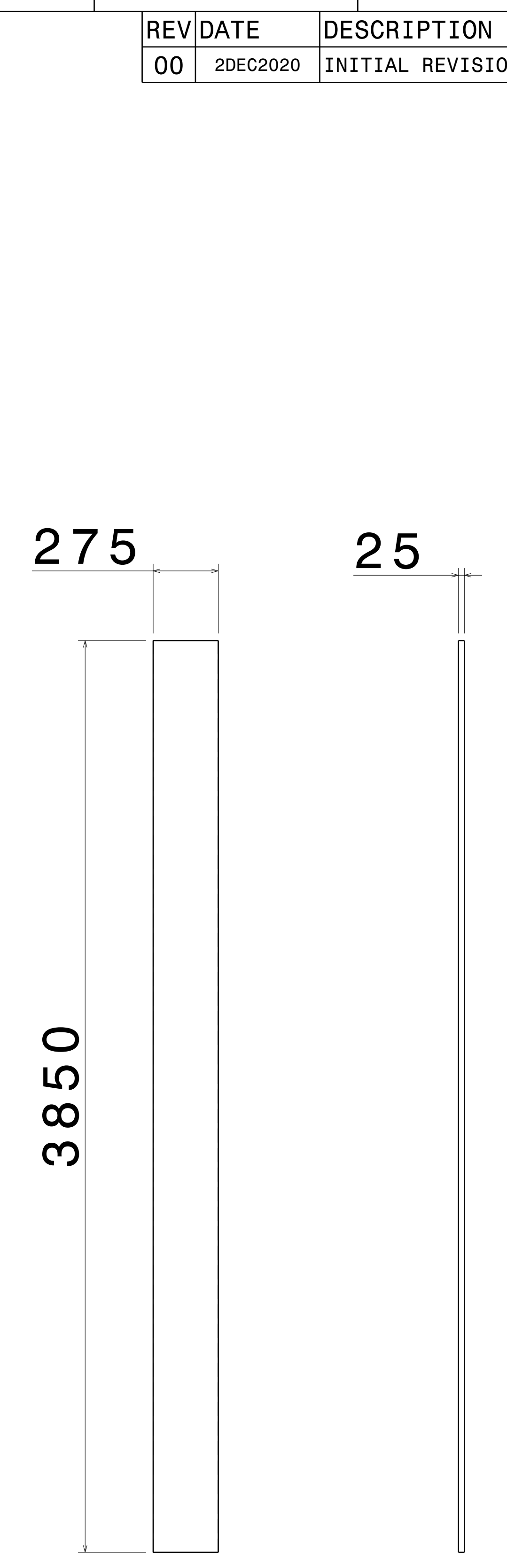
FRONT VIEW RIGHT VIEW SCALE: 1:15 SCALE: 1:15 ITEM 7, RHS PLANK 4 THICKNESS -1.6 MM
