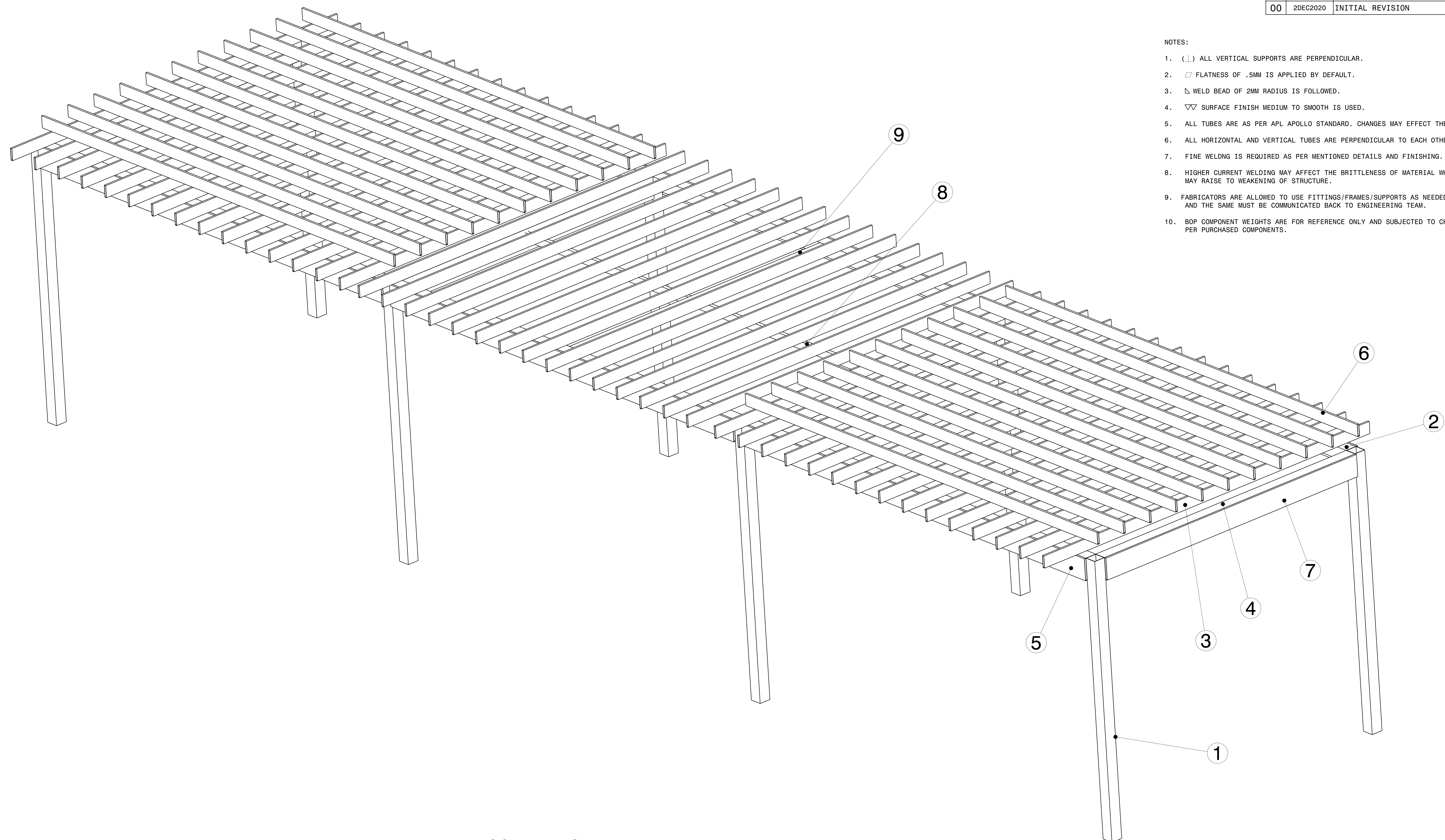
ISOMETRIC VIEW
