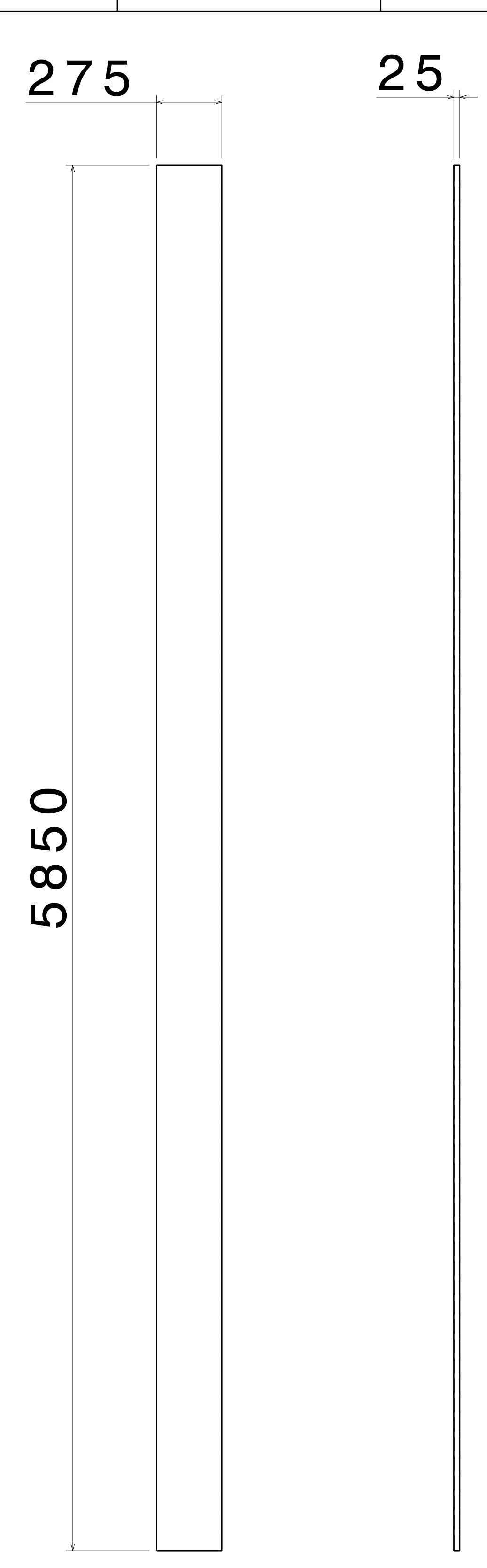
FRONT VIEW RIGHT VIEW SCALE: 1:15 SCALE: 1:15 ITEM 5, RHS PLANK 2 THICKNESS -1.6 MM
