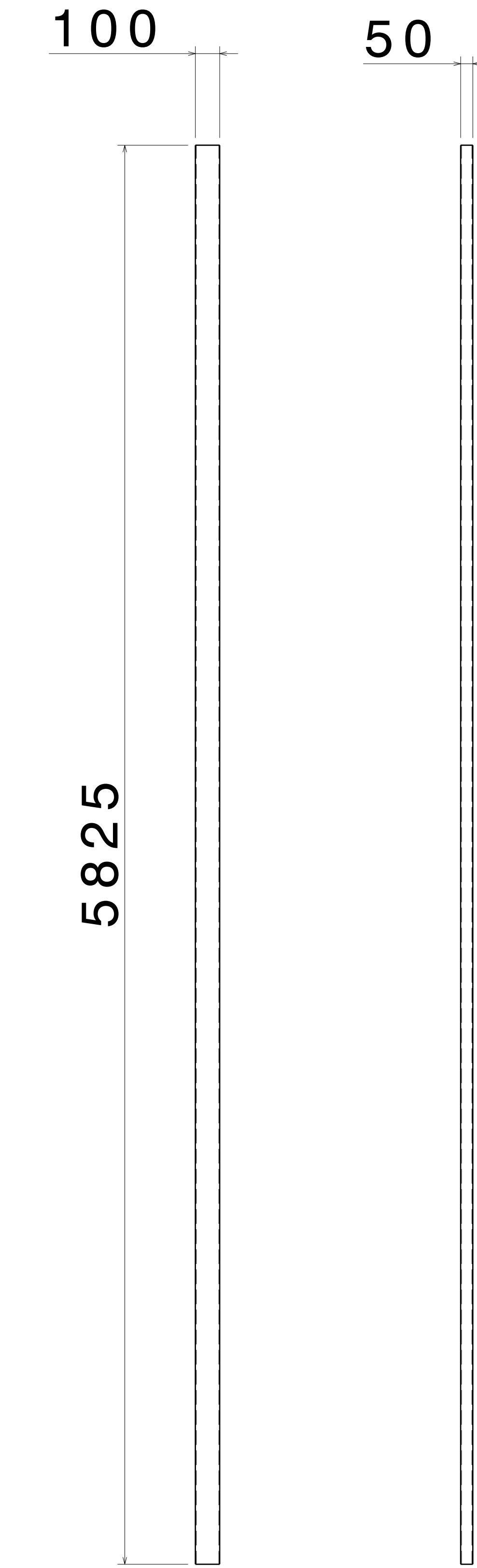
FRONT VIEW RIGHT VIEW SCALE: 1:15 SCALE: 1:15 ITEM 8, RHS FRAME 1 THICKNESS -3.6 MM
