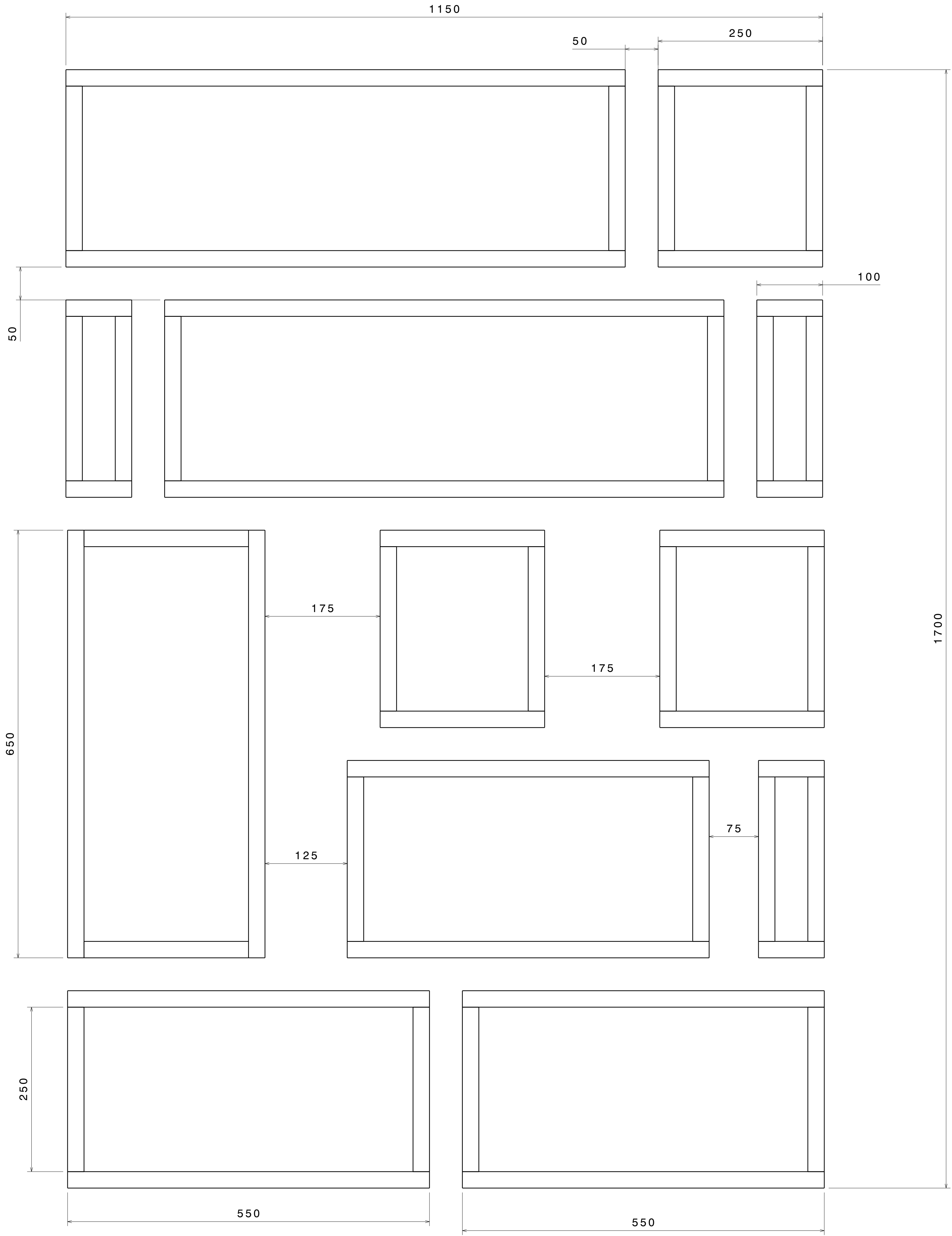
Front view Scale: 3:10
