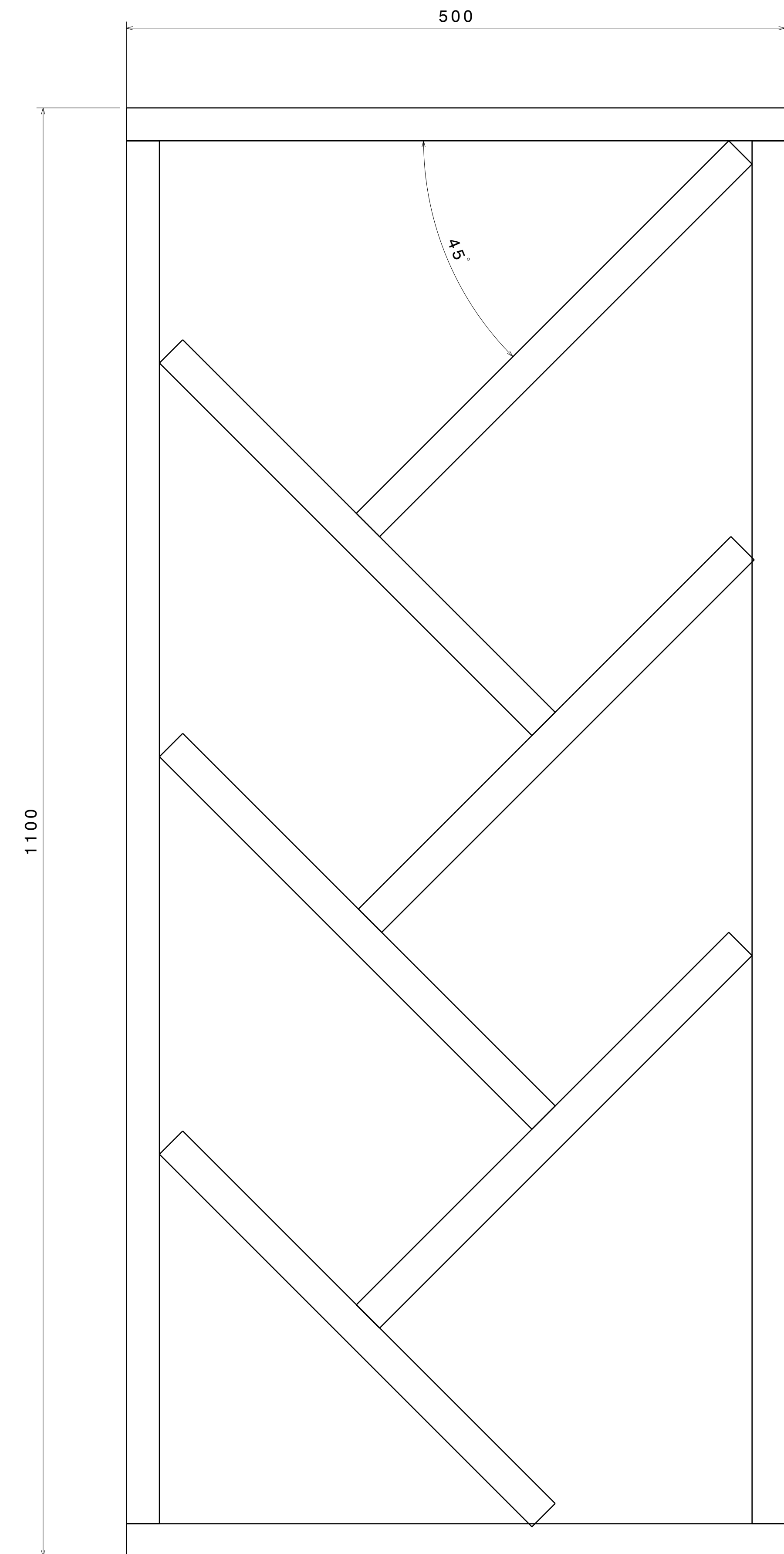
Front view Scale: 2:5
