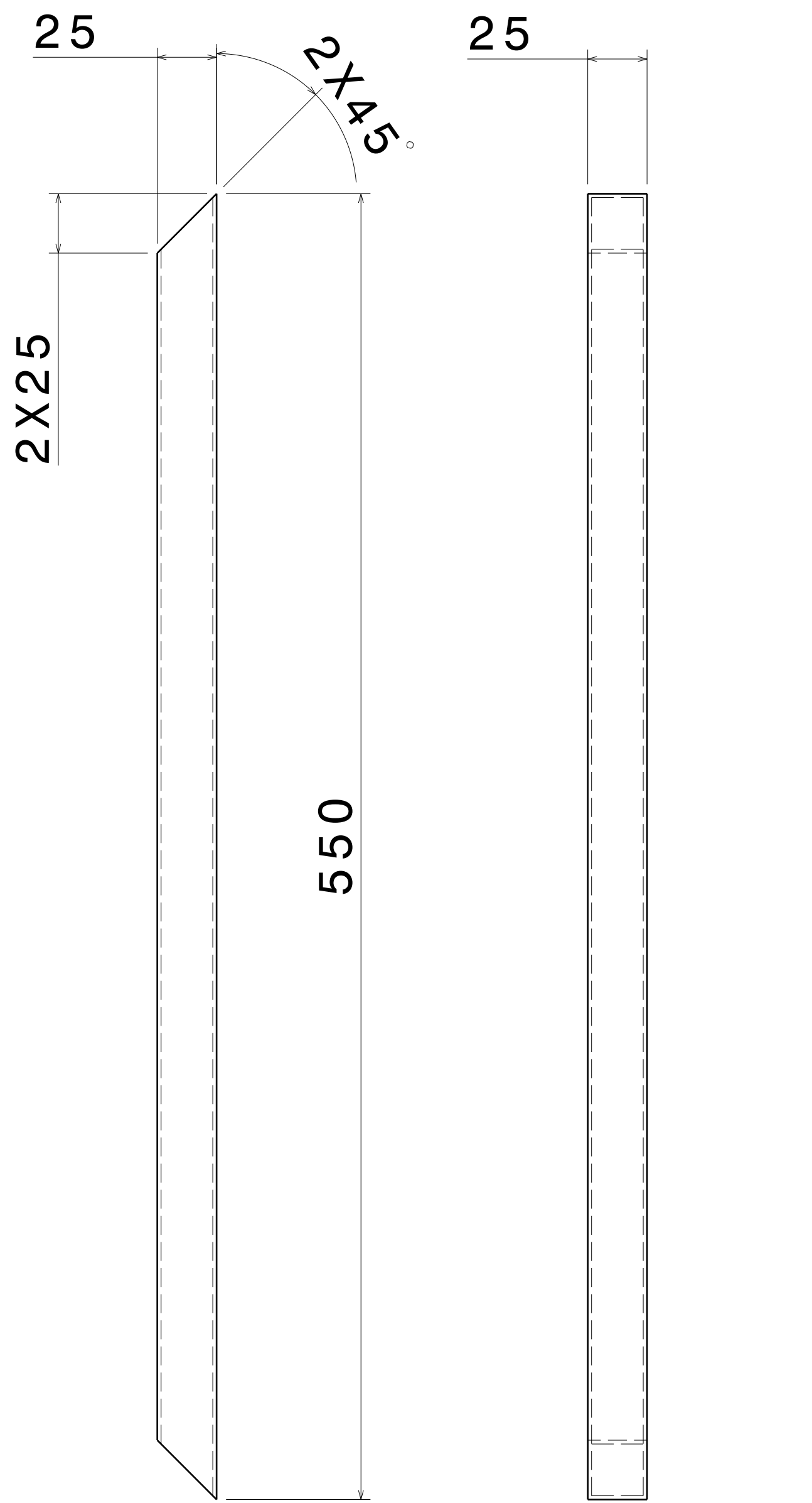
FRONT VIEW SCALE: 1:2 RIGHT VIEW SCALE: 1:2 ITEM 1, SHS FRAME 1 THICKNESS - 1.6MM
