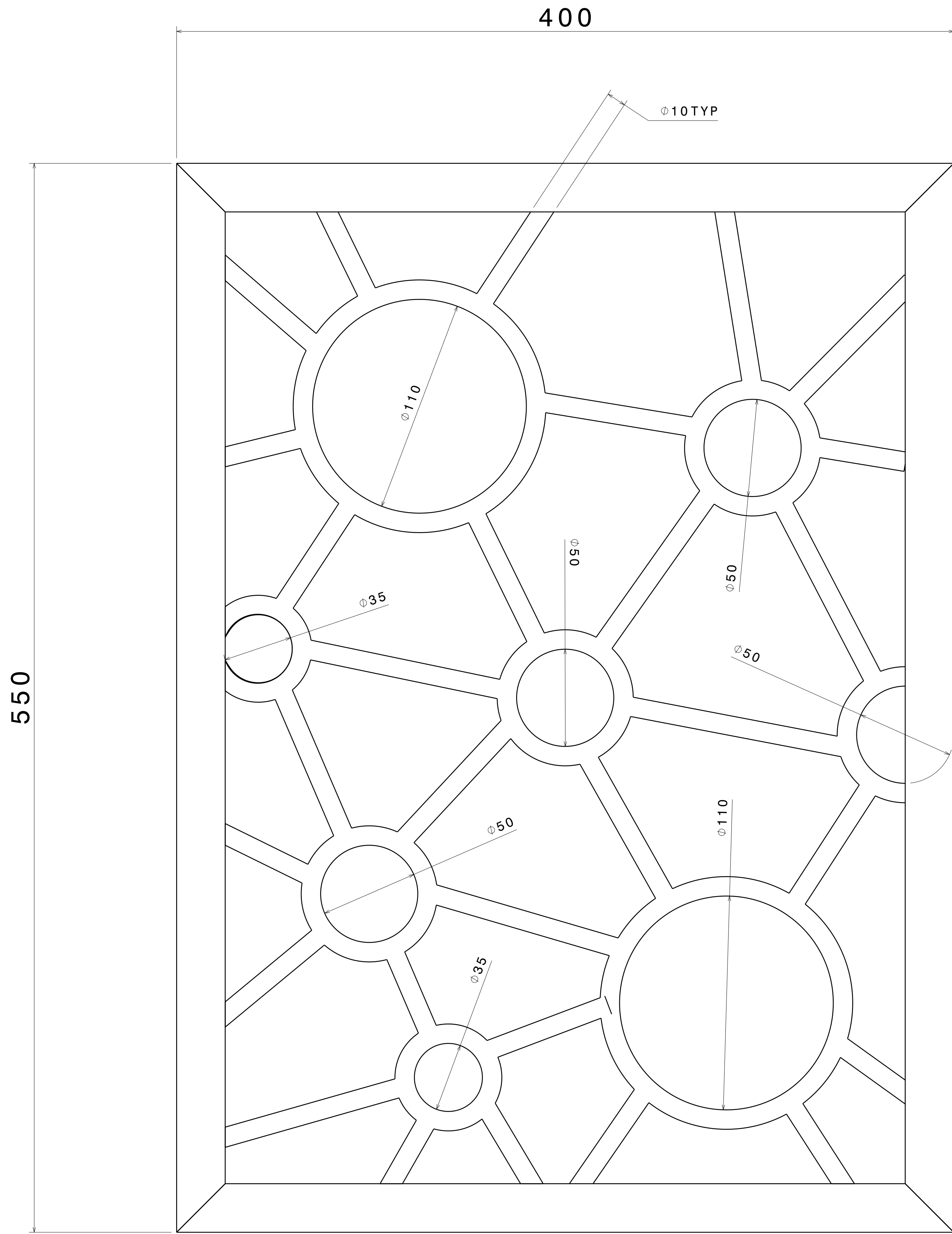
FRONT VIEW
