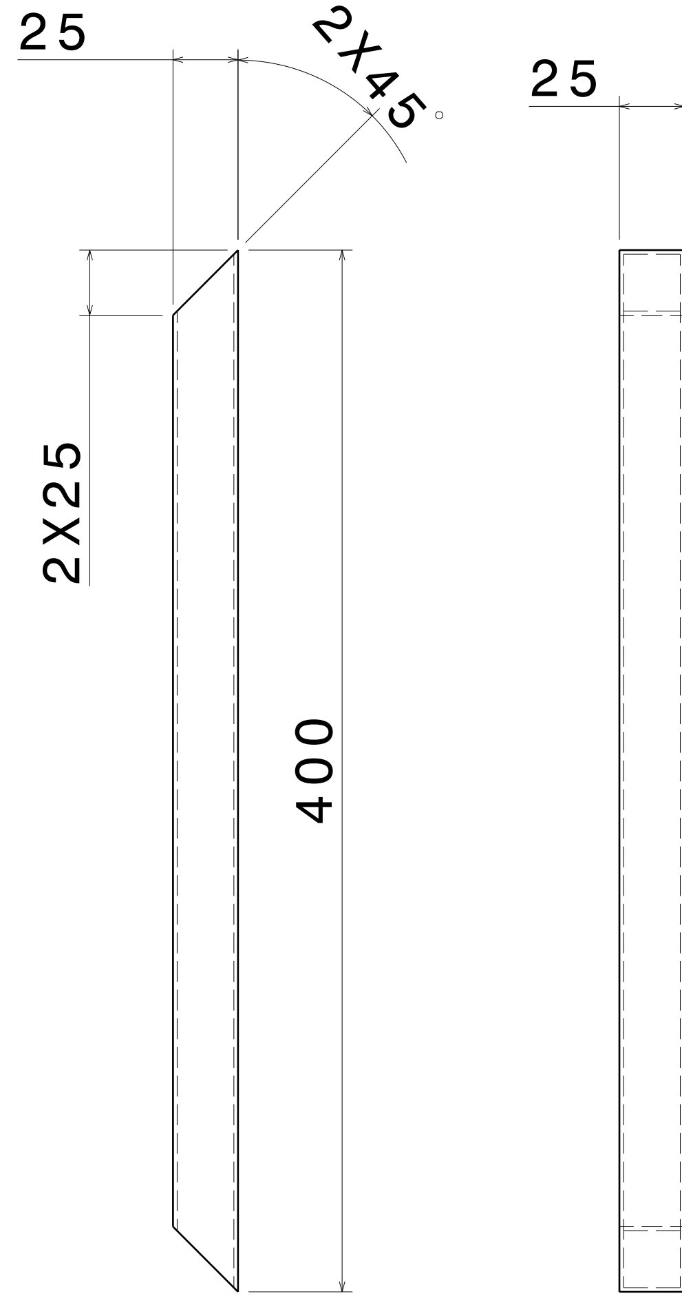
FRONT VIEW SCALE: 1:2 RIGHT VIEW SCALE: 1:2 ITEM 2, SHS FRAME 2 THICKNESS - 1.6MM
