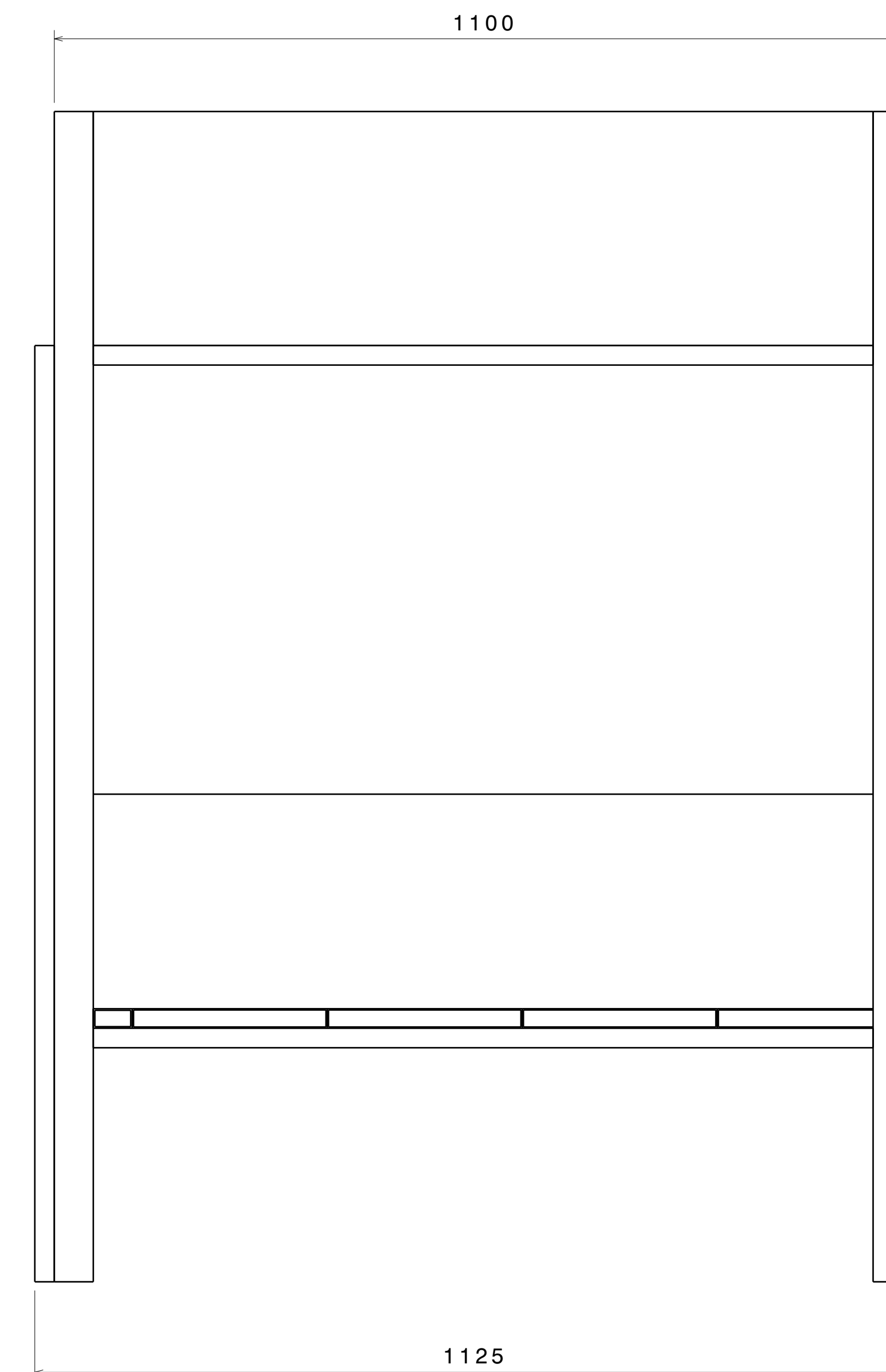
Right view
