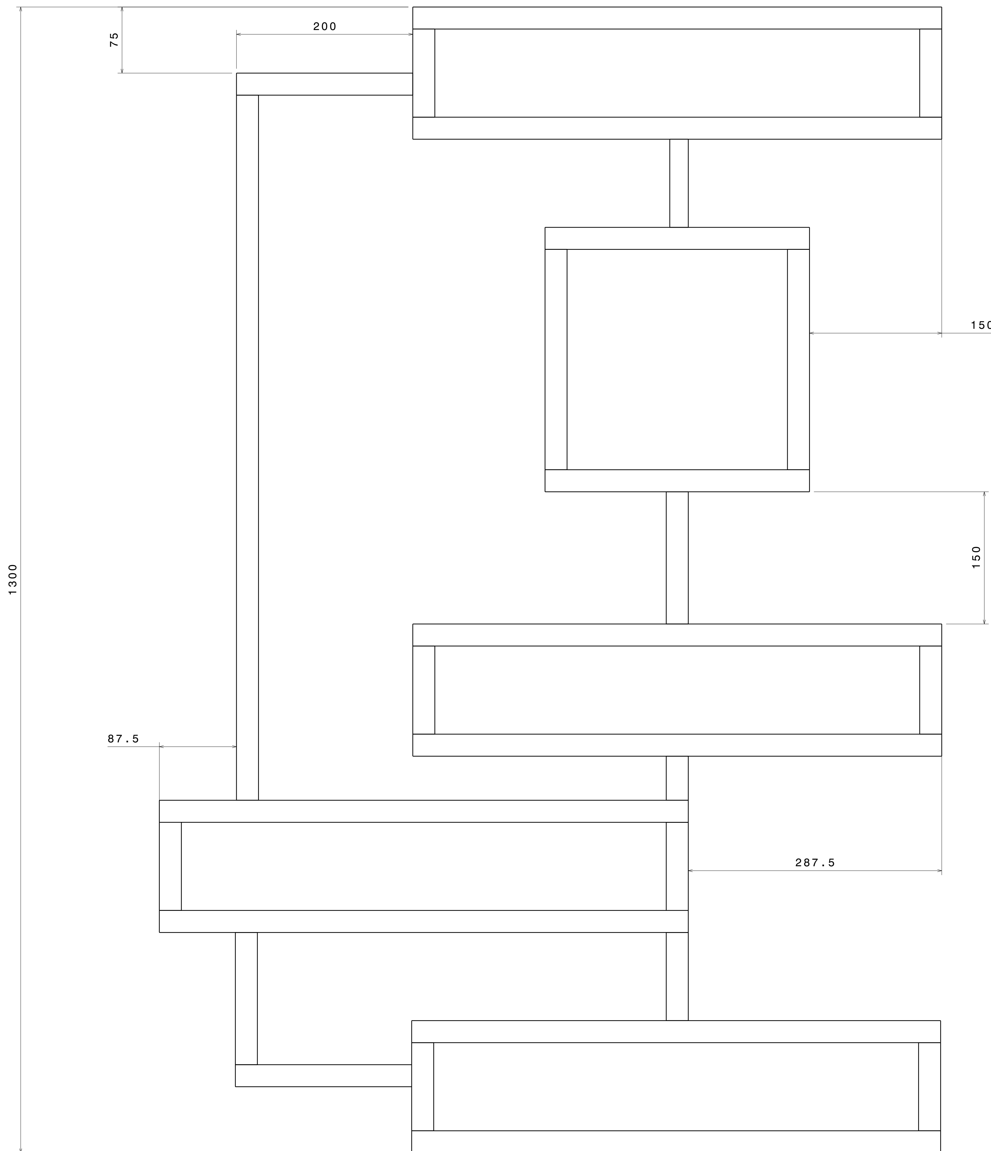
Front view Scale: 2:5
