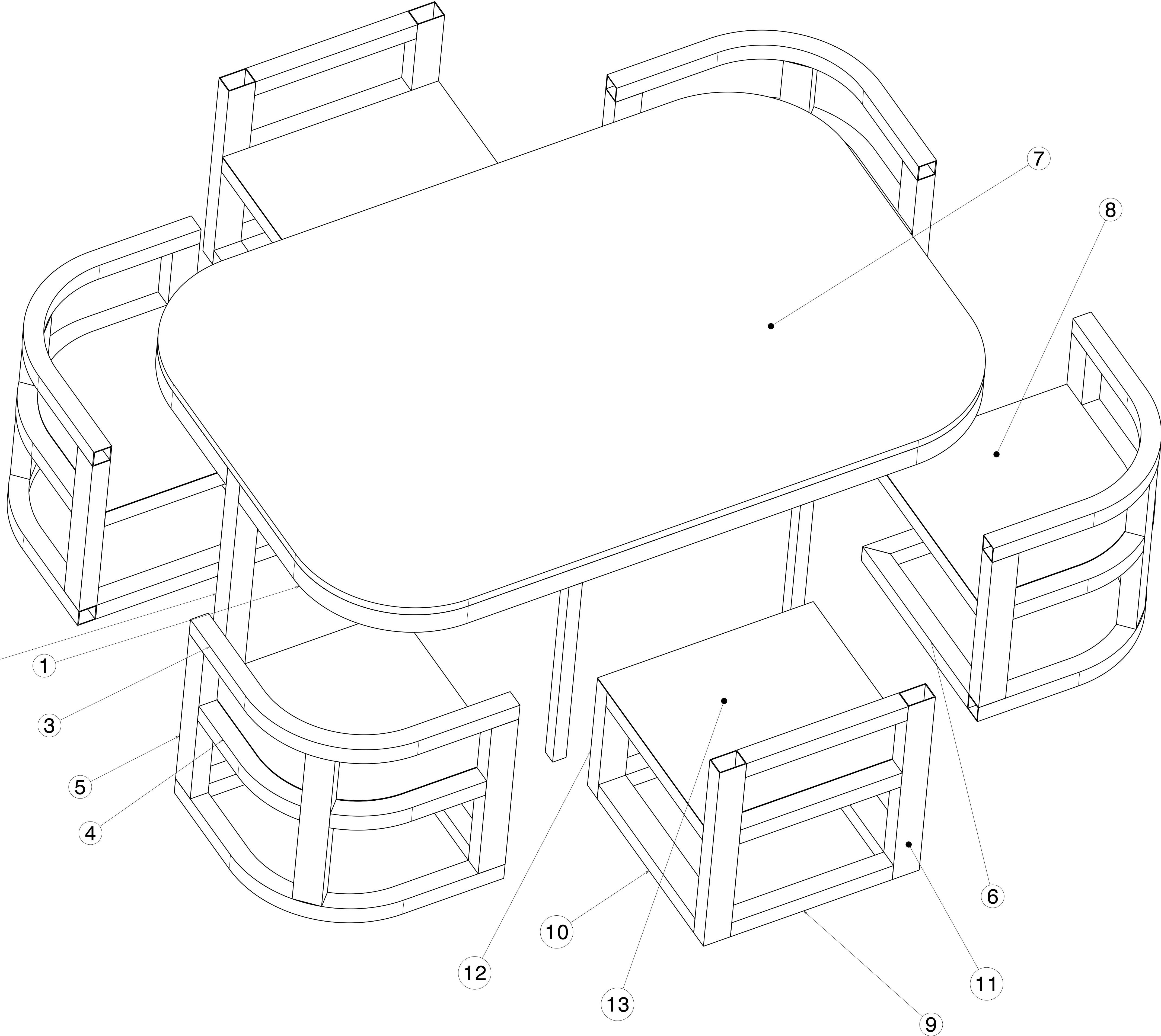
Isometric view EXPLODED
