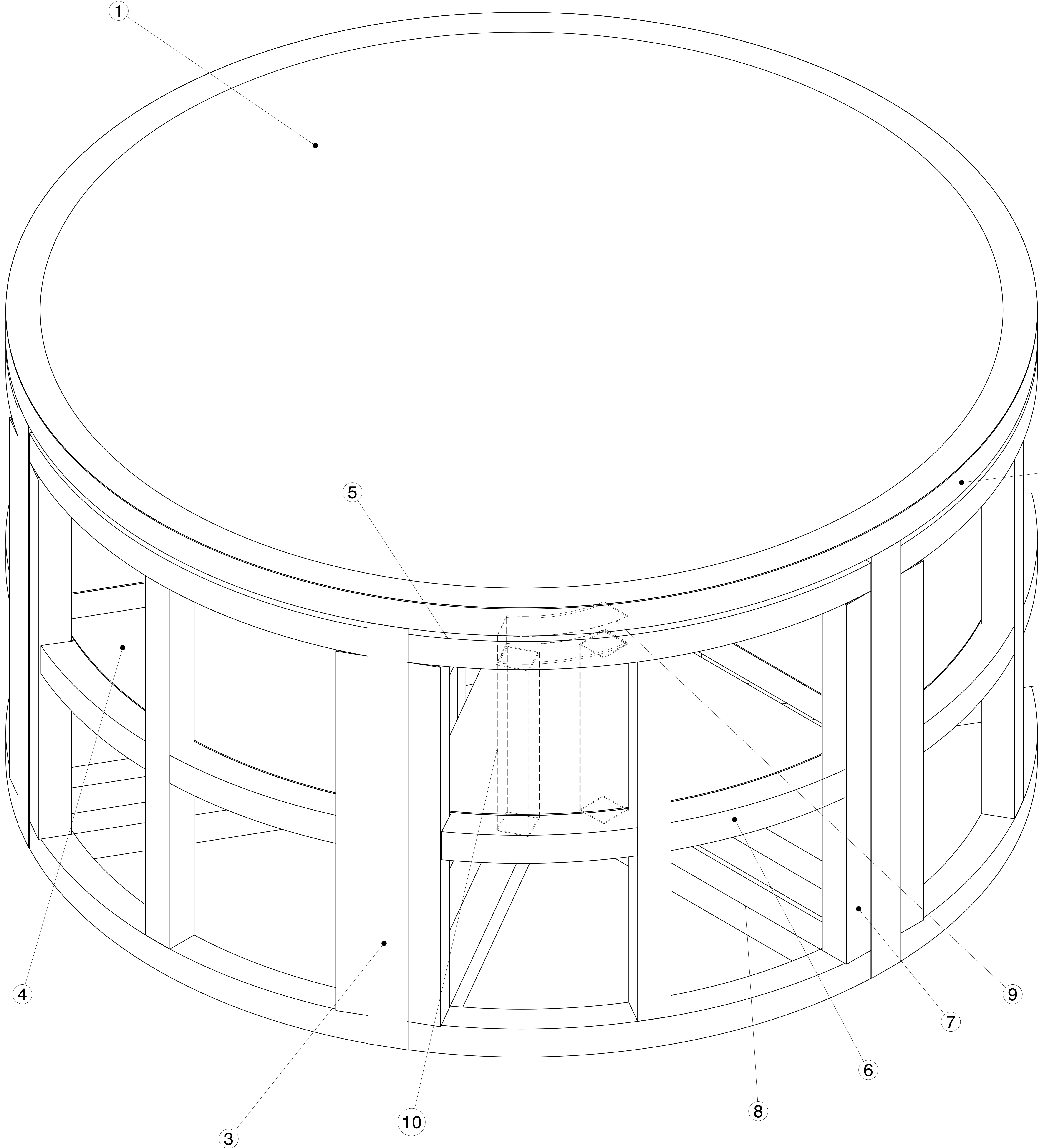
Isometric view Scale: 2:5
