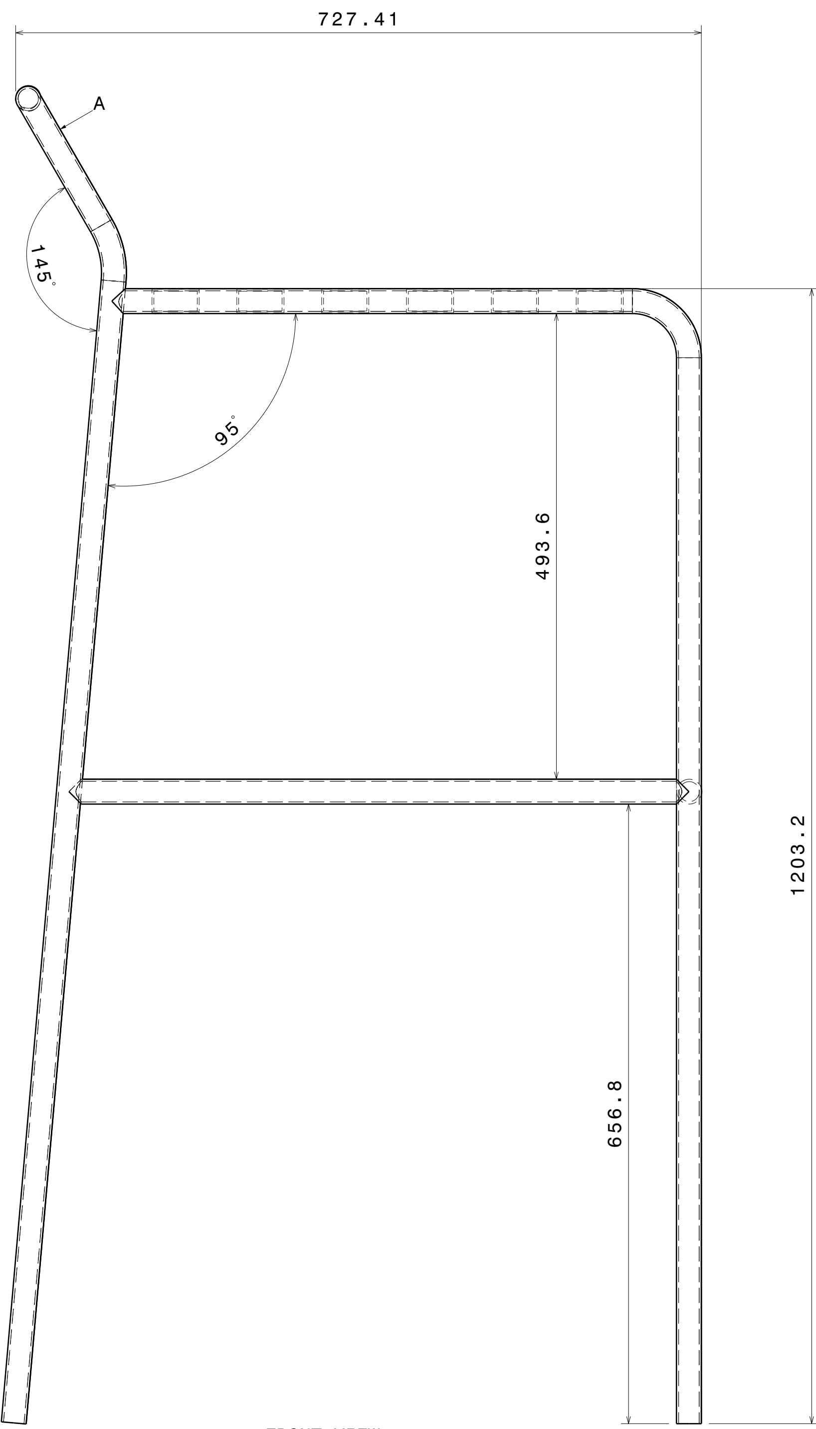
FRONT VIEW, CHAIR 1
