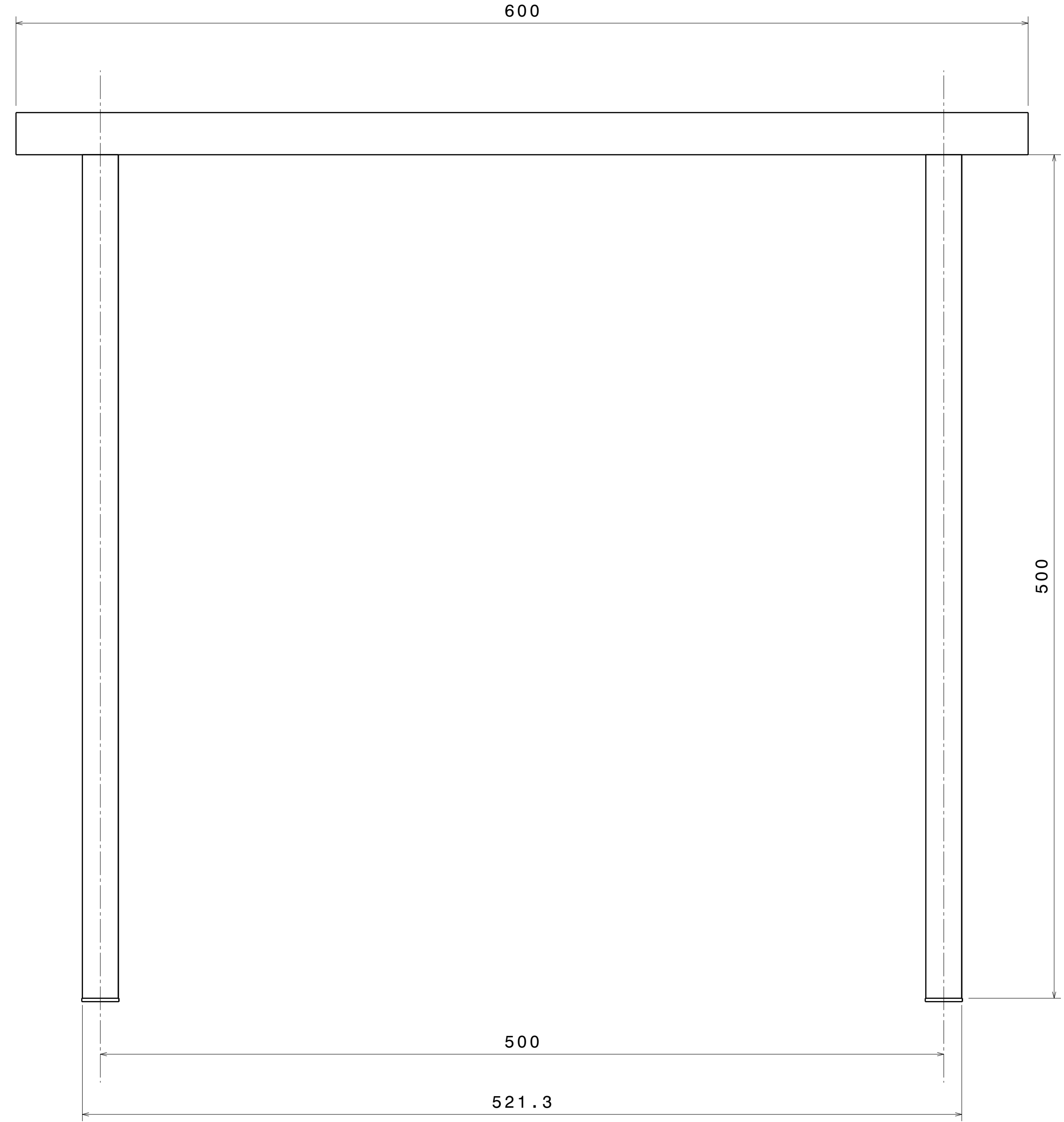
Front view Scale: 1:2
