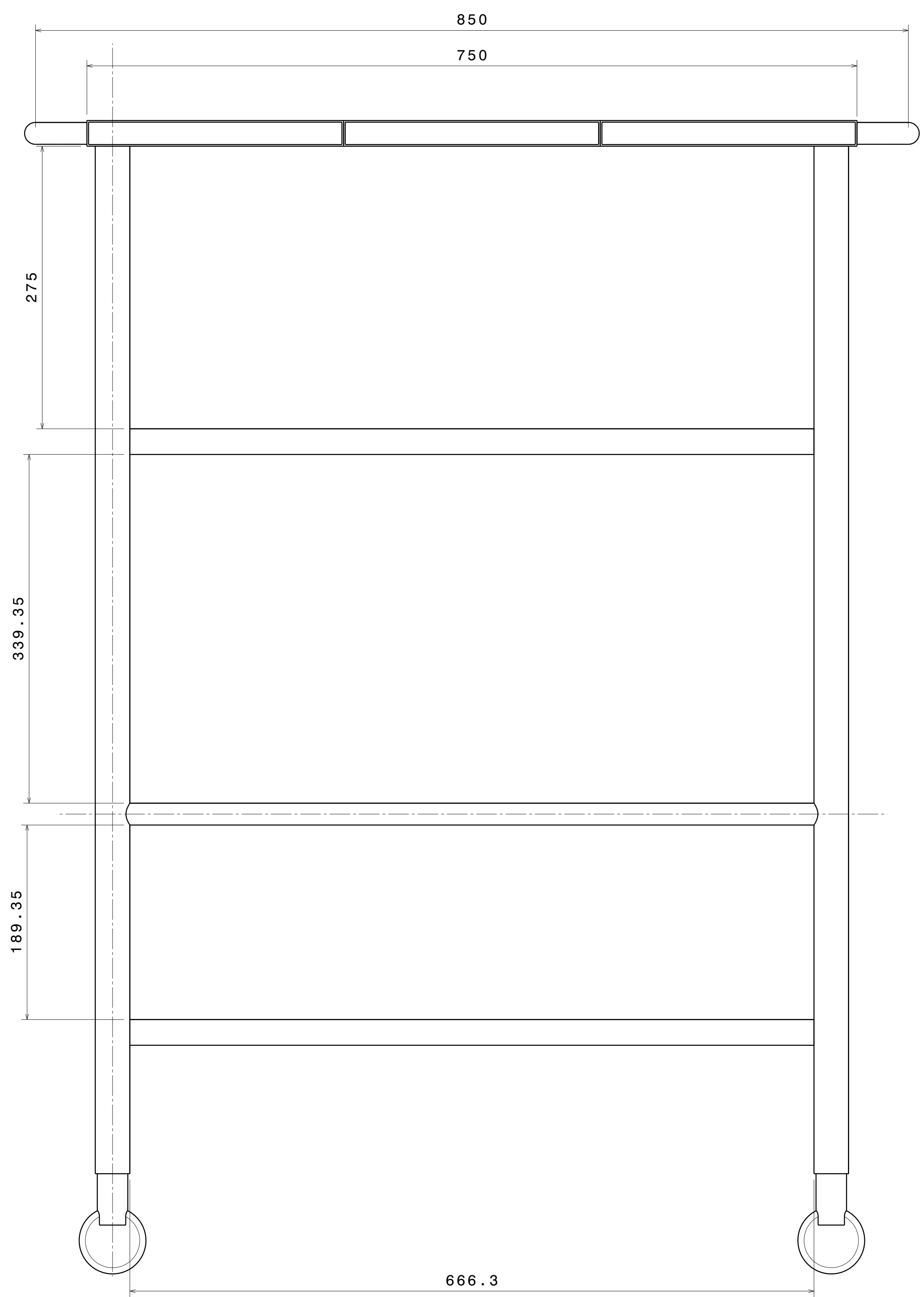
Front view Scale: 7:20
