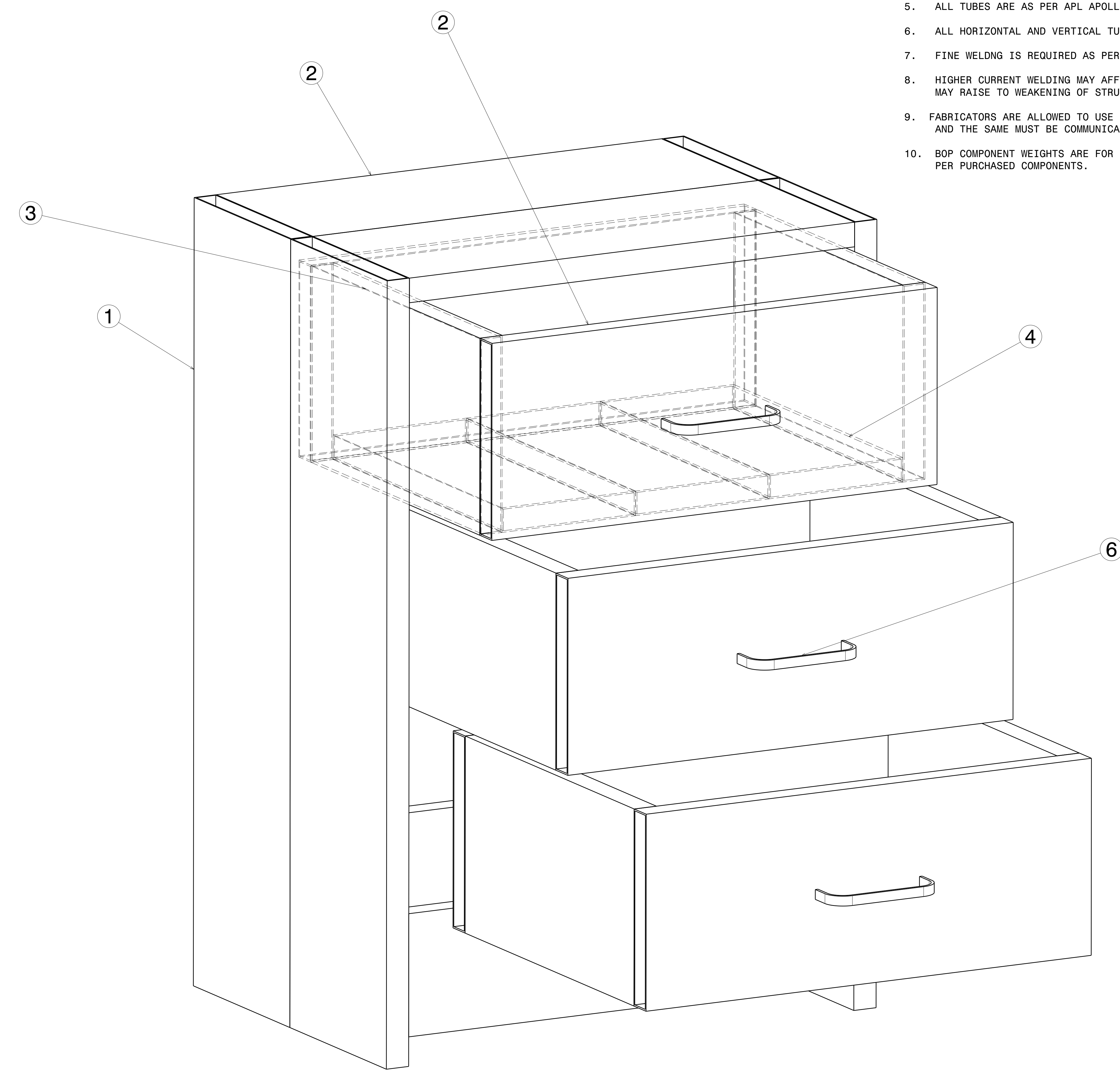
EXPLODED VIEW
