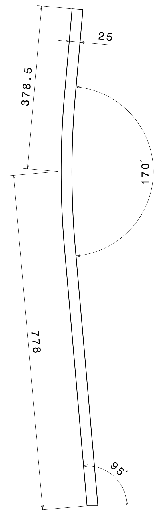
ITEM 2 DETAILS Rect Tube Chair & Table Frame 2
