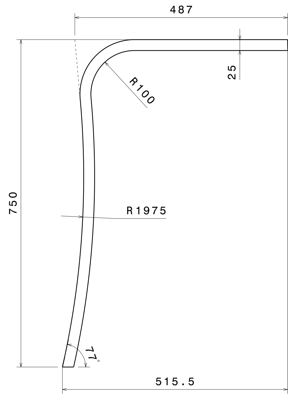
ITEM 1 DETAILS Rect Tube Chair & Table Frame 1
