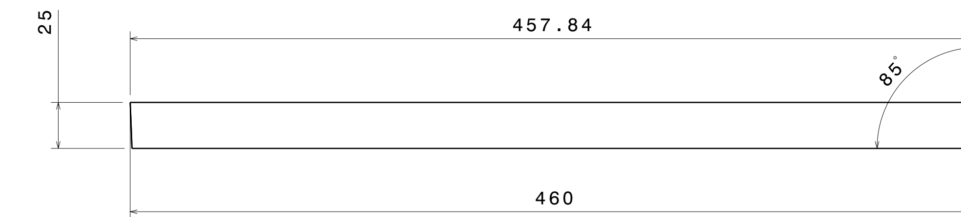
ITEM 3 DETAILS Rect Tube Chair & Table Frame 3
