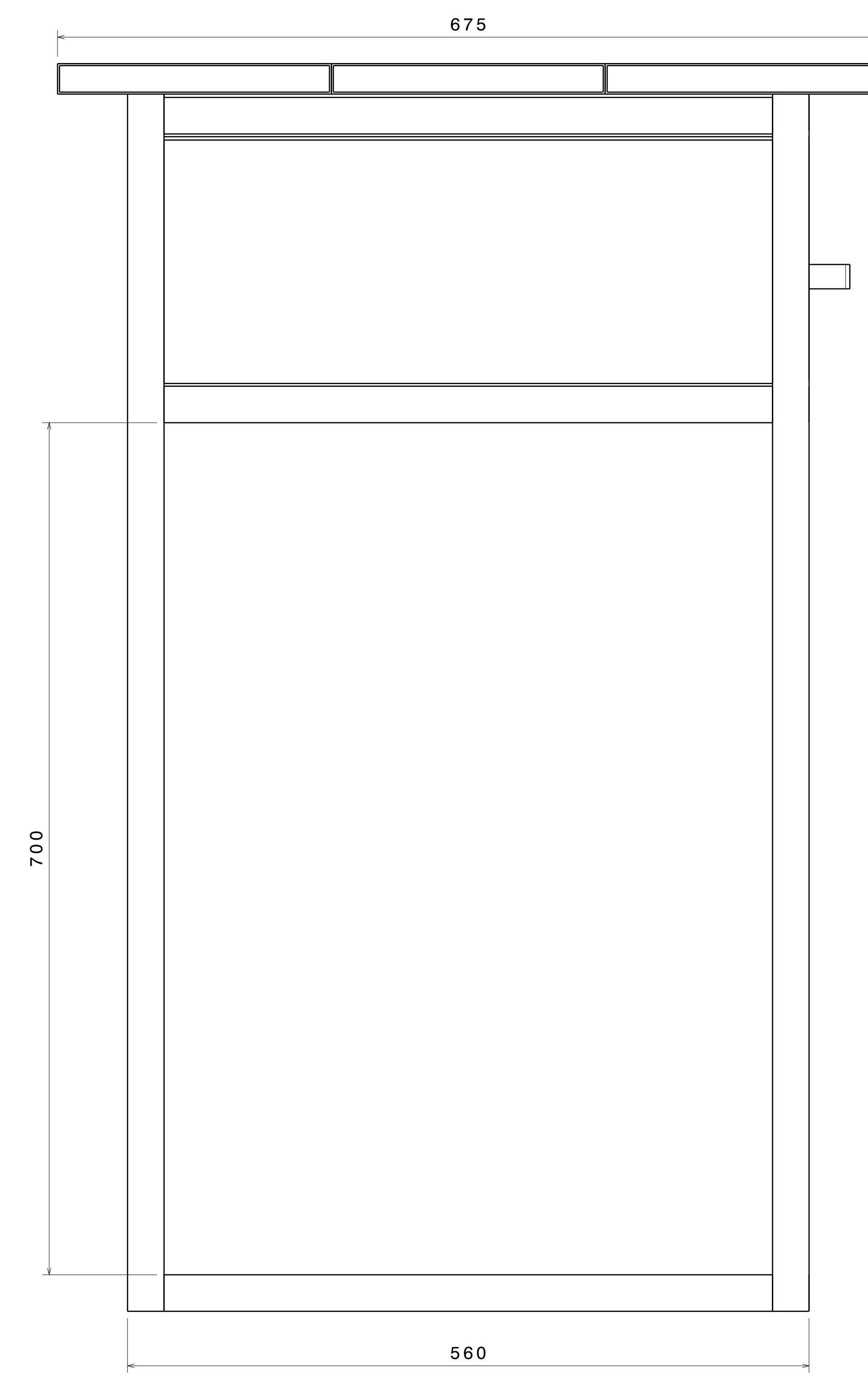
Front view Scale: 7:20
