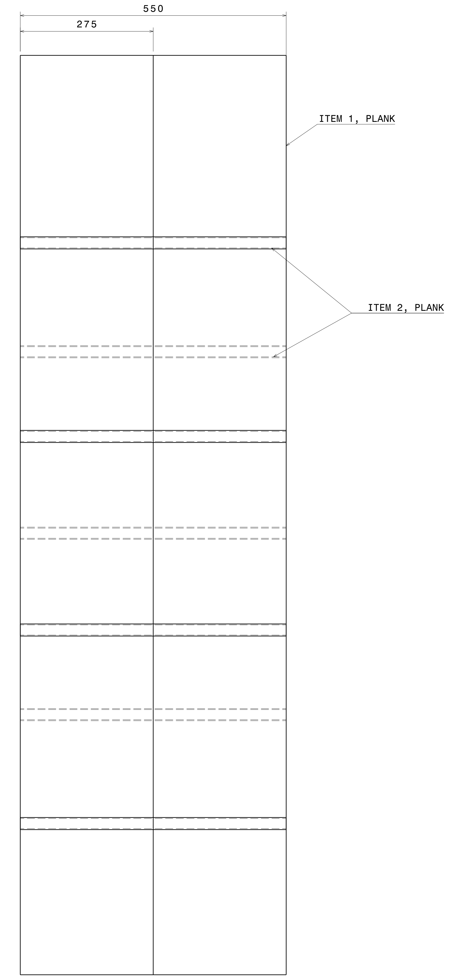
Right view Scale: 1:4 WALLS ARE OMITTED FOR CLARITY
