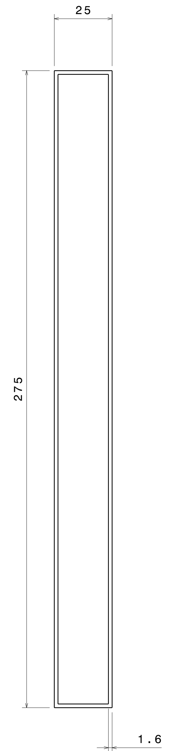
TYPICAL CROSS SECTION VIEW FOR ITEMS 3, 4, 5, 6, 7, 8, 9, 10, 11
