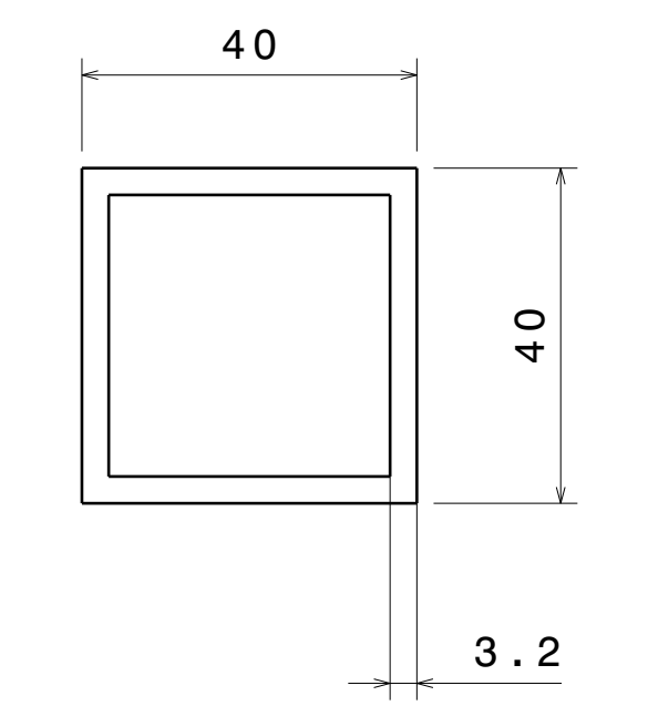
Section Detail of ITEM 3 & 5 Scale: 1:1
