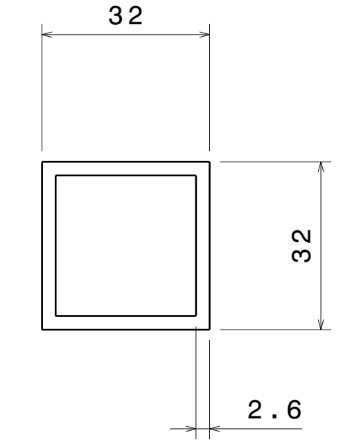
Section Detail of ITEM 6 Scale: 1:1
