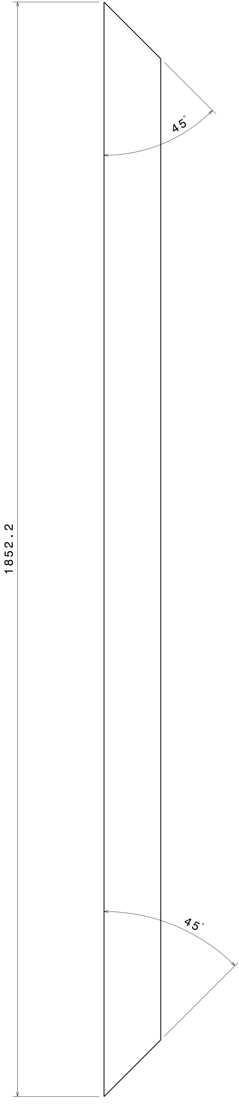
ITEM 1 DETAILS rect_tube 36.1 Frame 1
