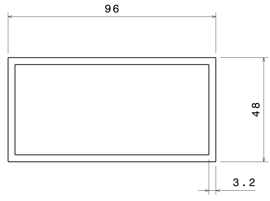
Section Detail of ITEM 1 & 2 Scale: 1:1
