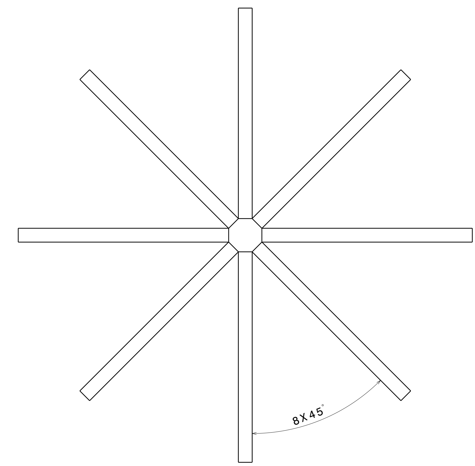
ITEM 47, QTY 8, WELDED TOGETHER AS SHOWN SIZE: 25 X 25 X 1.6 X 380
