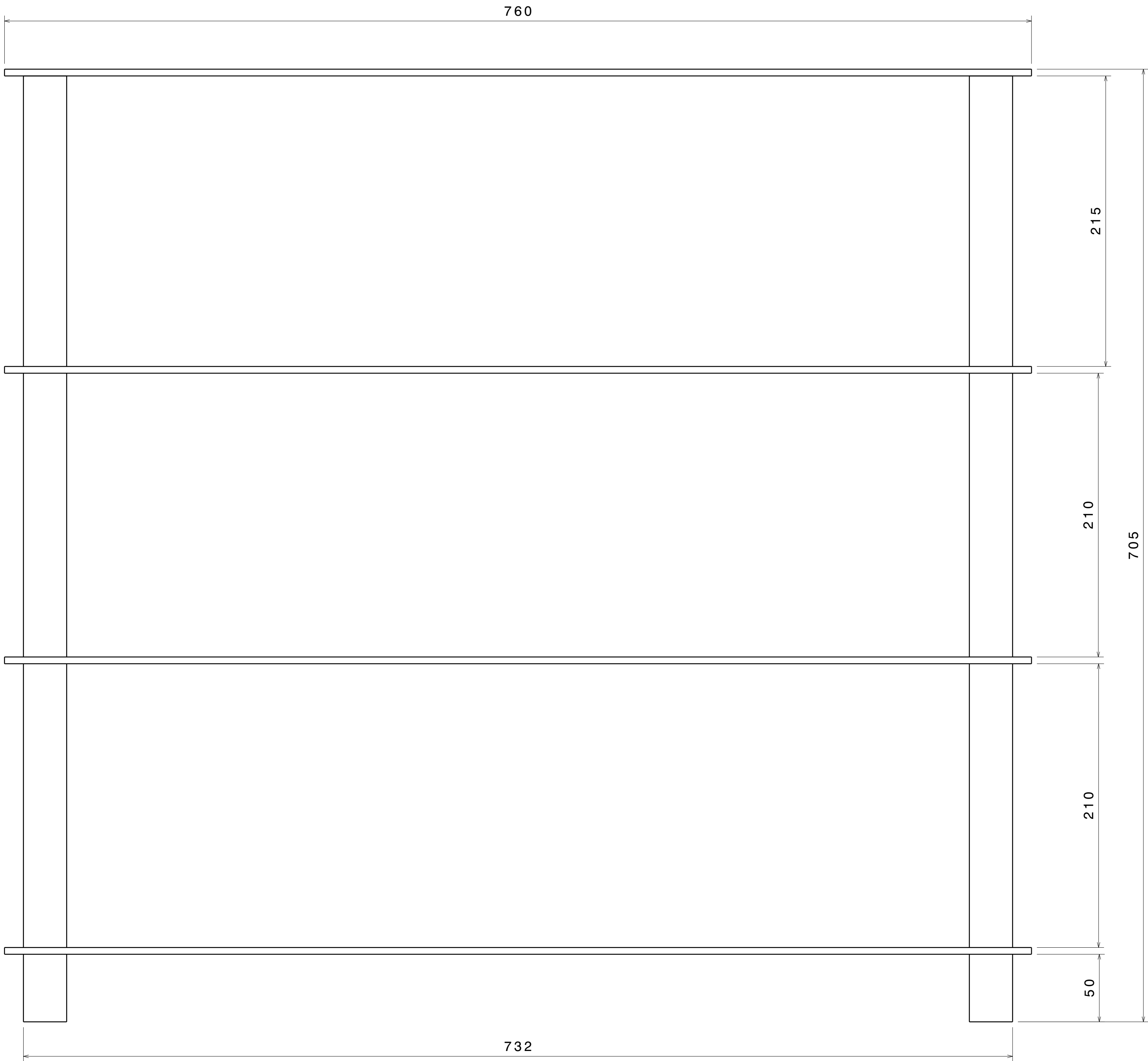
Front view Scale: 1:2
