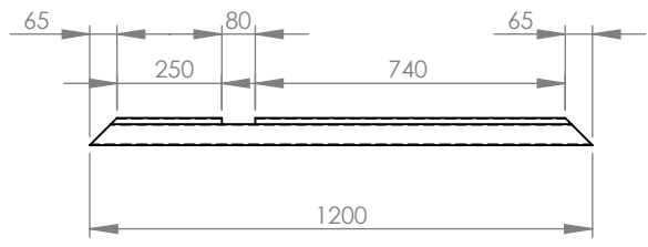
ITEM 1 DDF 130X65X2.0X1200
