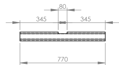
ITEM 6 FDF 130X80X2.0X770
