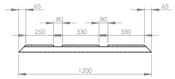
ITEM 3 DDF 130X65X2.0X1200 (2)
