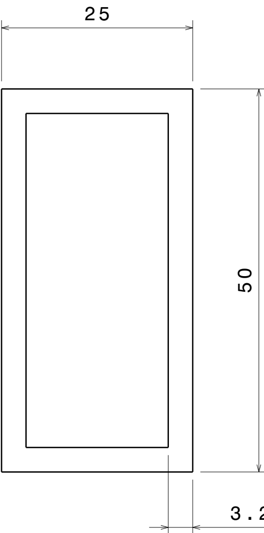
Section Detail of ITEM 5 & 9 Scale: 2:1
