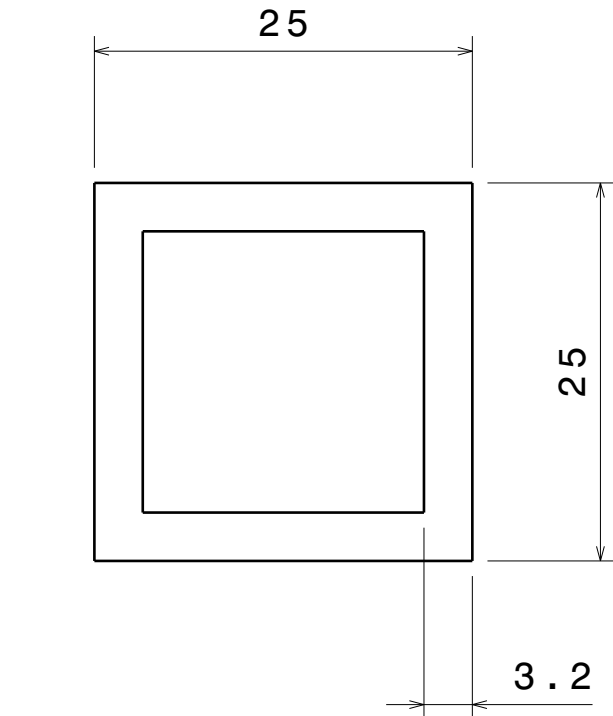
Section Detail of ITEM 1,2 & 8 Scale: 2:1
