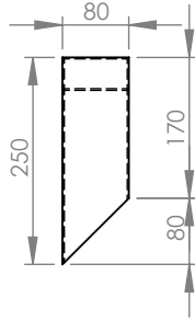
ITEM 1 RHS 80X40X2.0X250
