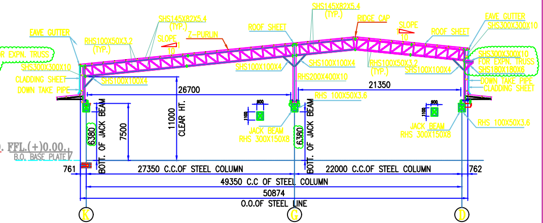
CROSS SECTION ALONG GRID- 2
