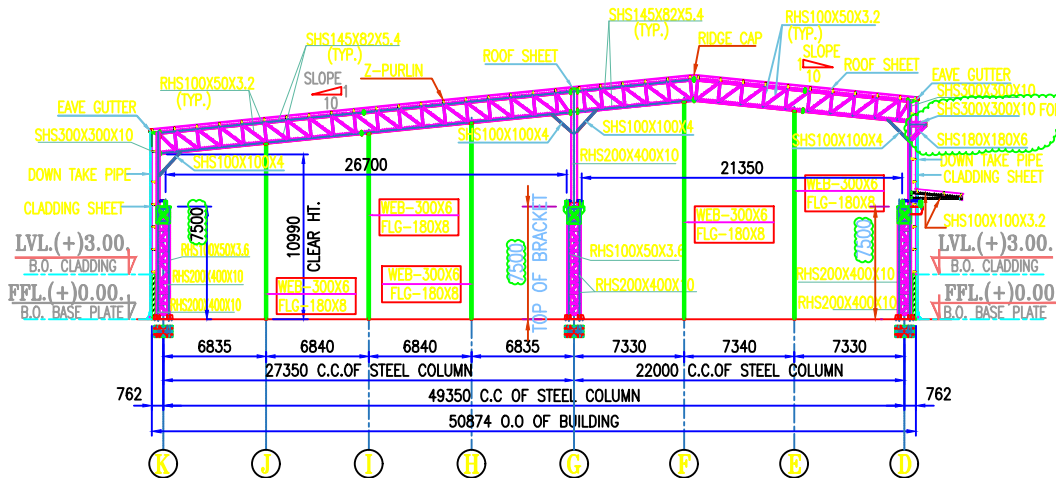
CROSS SECTION ALONG GRID-1
