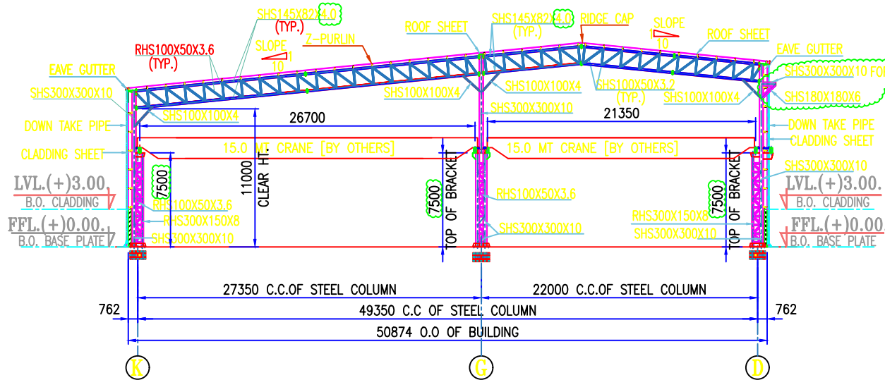
CROSS SECTION ALONG GRID-6 TO 19
