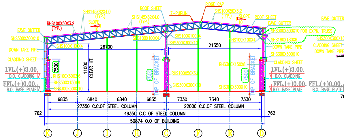
CROSS SECTION ALONG GRID-20
