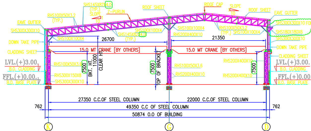
CROSS SECTION ALONG GRID-5 &amp; 3
