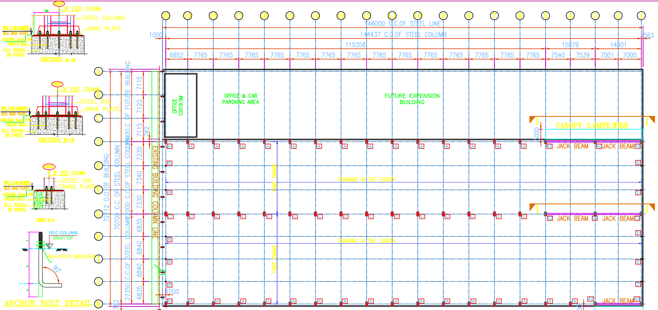
ANCHOR BOLT PLAN
