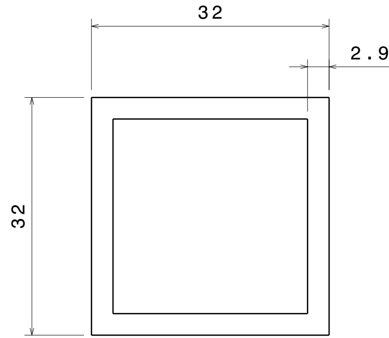
Section Detail of ITEM 1,2,3,4,5 & 6 Scale: 2:1
