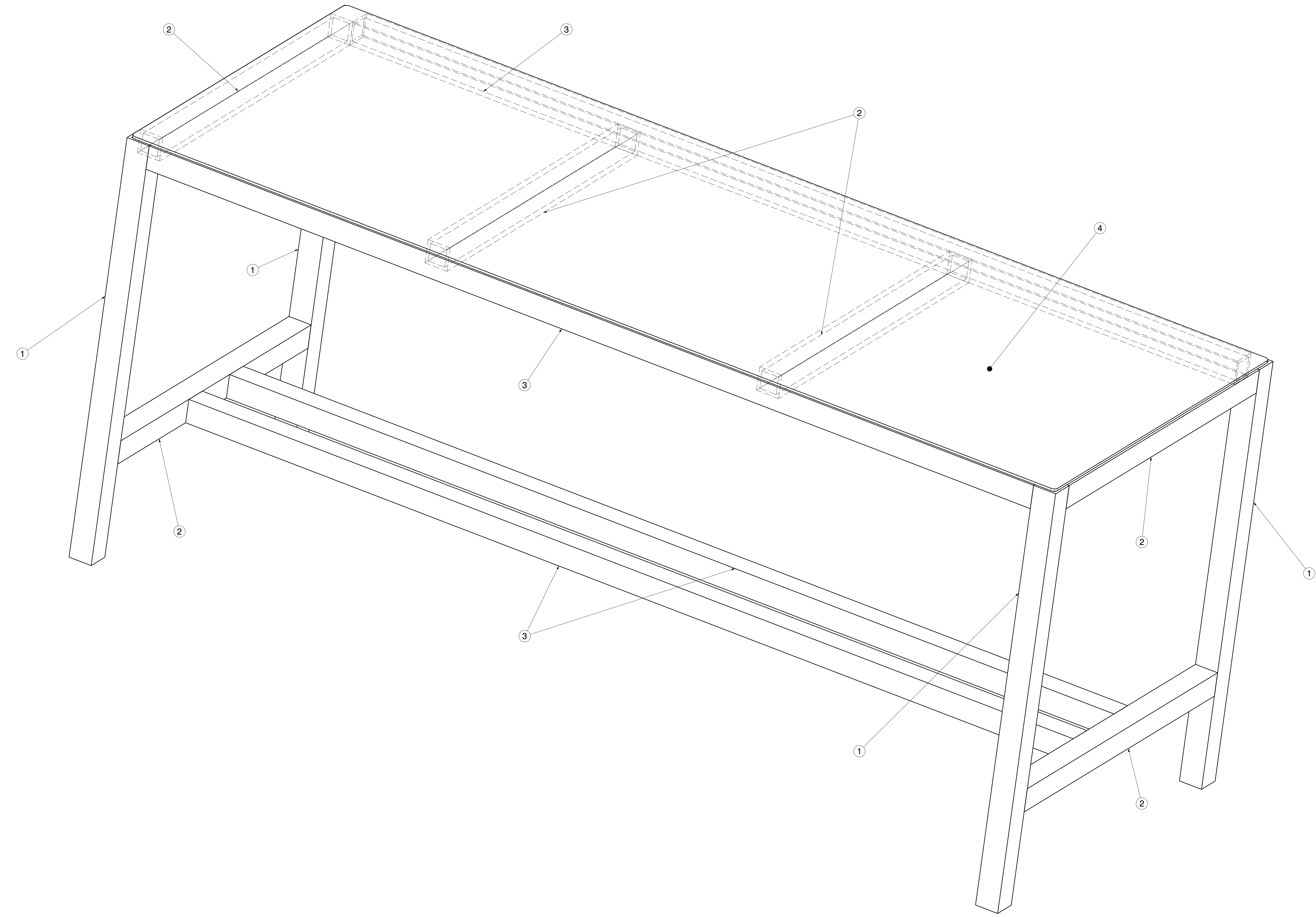
Isometric view
