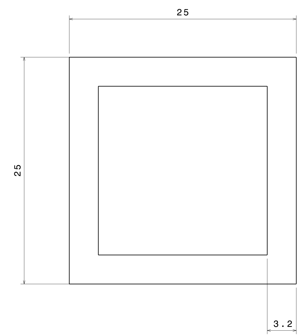
Section Detail of ITEM 1, 2 & 3 Scale: 5:1
