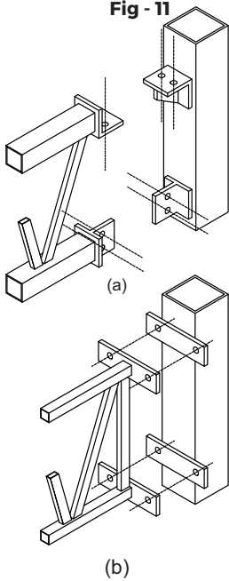
Figure 11(a&b) - Truss to SHS/RHS column connection
