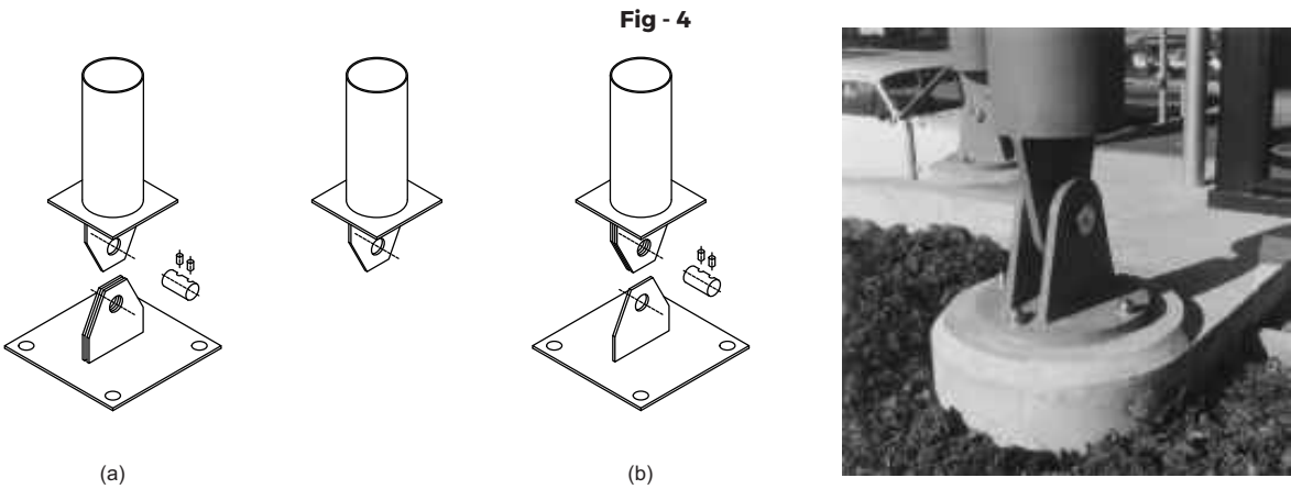
Some examples of tubular connections with pinned ends
